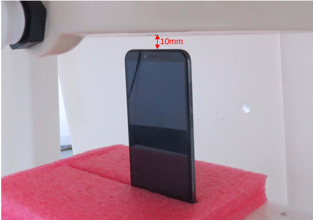
Picture 11: Top Side, the distance from handset to the bottom of the Phantom is 10mm (ATU-L11)
