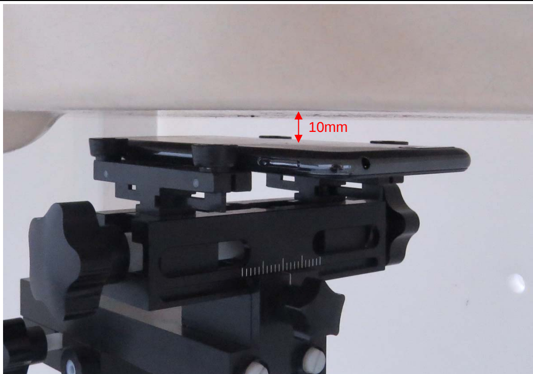
Picture 7: Back Side, the distance from handset to the bottom of the Phantom is 10mm (ATU-L11)
