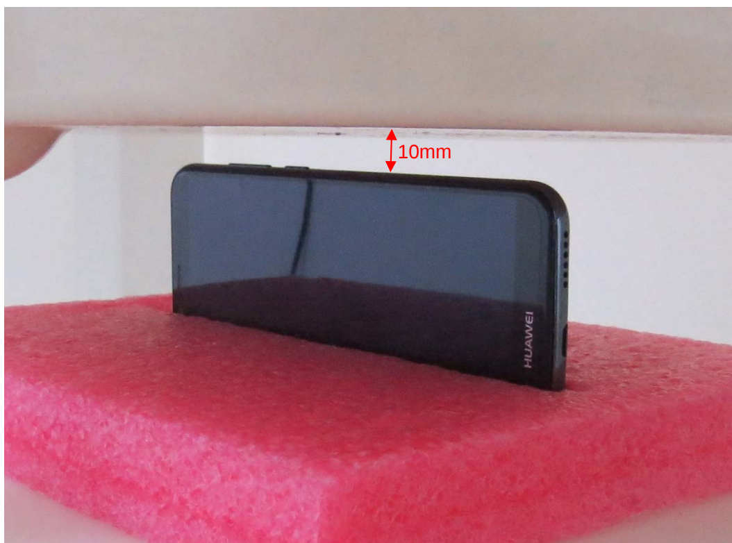
Picture 10: Right Side, the distance from handset to the bottom of the Phantom is 10mm (ATU-L11)
