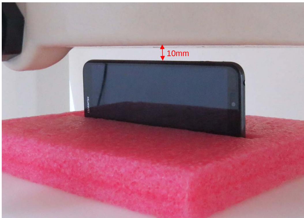
Picture 9: Left Side, the distance from handset to the bottom of the Phantom is 10mm (ATU-L11)
