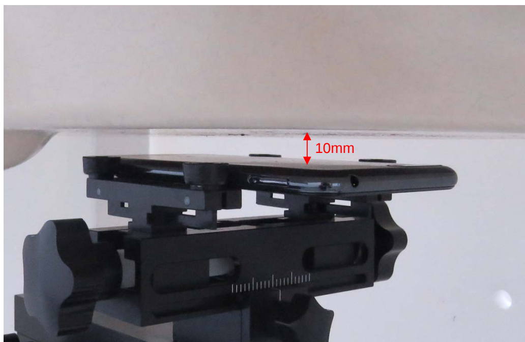
Picture 16: Back Side, the distance from handset to the bottom of the Phantom is 10mm (ATU-L21)
