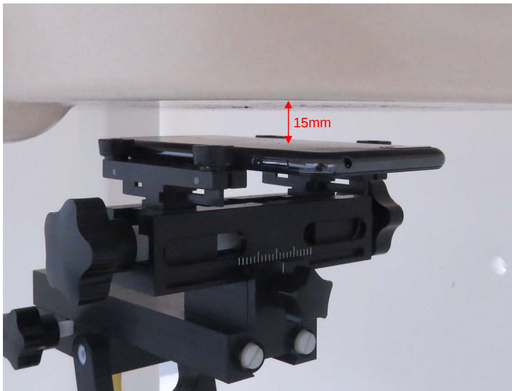
Picture 15: Back Side, the distance from handset to the bottom of the Phantom is 15mm (ATU-L21)
