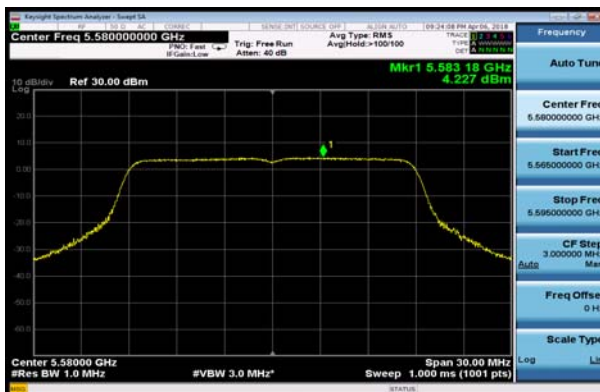
U-NII-2C, 802.11n HT20, Channel No.: 116
