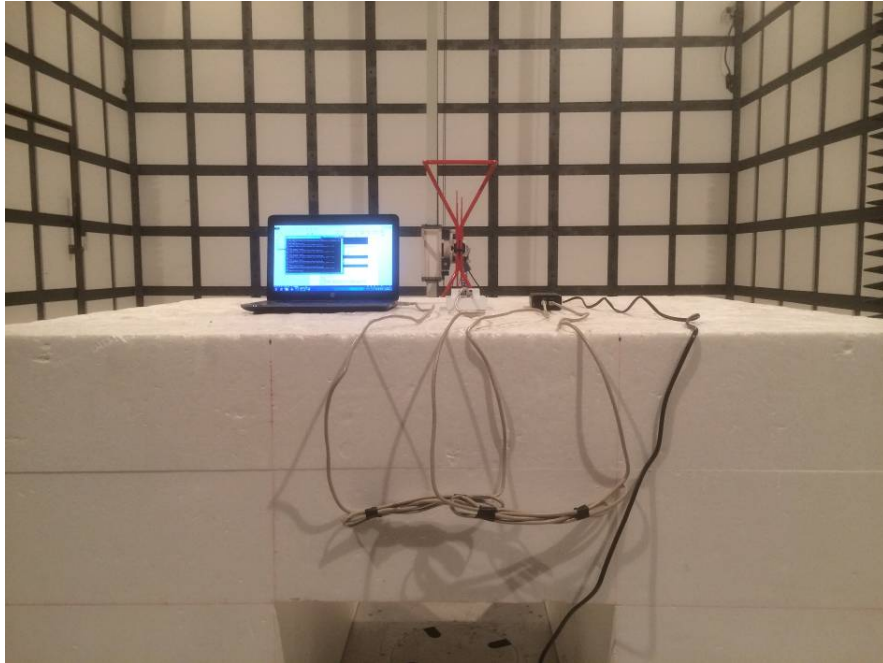
RSE – Rear View (Above 1 GHz)
