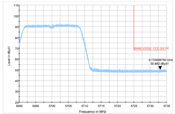
802.11ac HT20 -Channel 140: Peak
