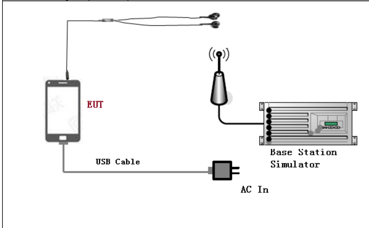
Connection Diagram (Mode 2~4)
