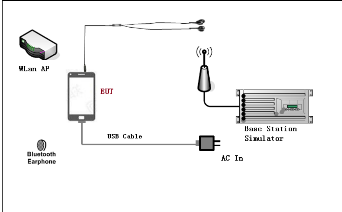
Connection Diagram (Mode 1)
