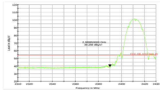
802.11b-Channel 1 Average
