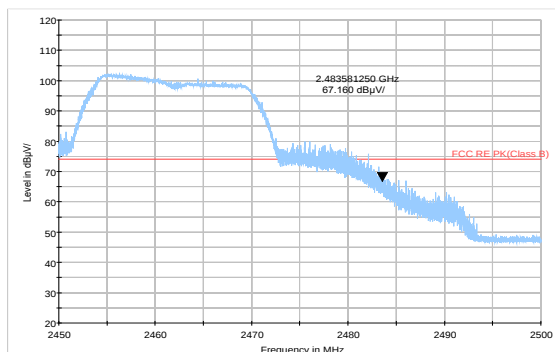
802.11g-Channel 11 Peak
