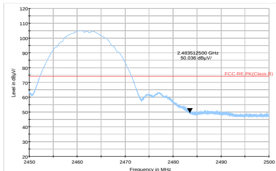
802.11b-Channel 11 Peak
