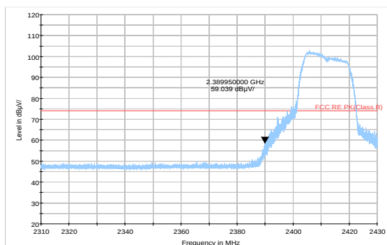
802.11g-Channel 1 Peak
