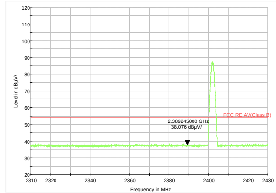
BLE V 5.0 Channel 0 Average
