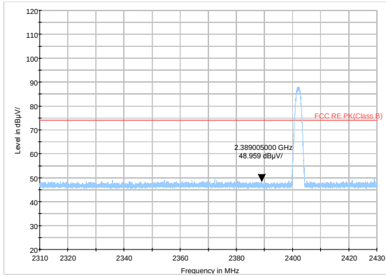
BLE V 5.0 Channel 0 Peak
