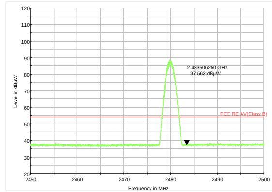
BLE V 5.0 Channel 39 Average
