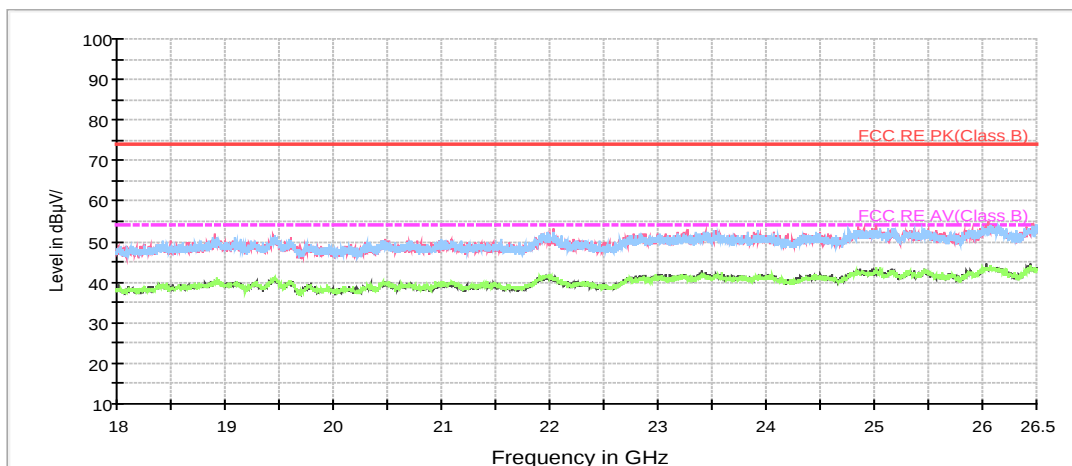
RE 18-26.5GHz PK+AV
