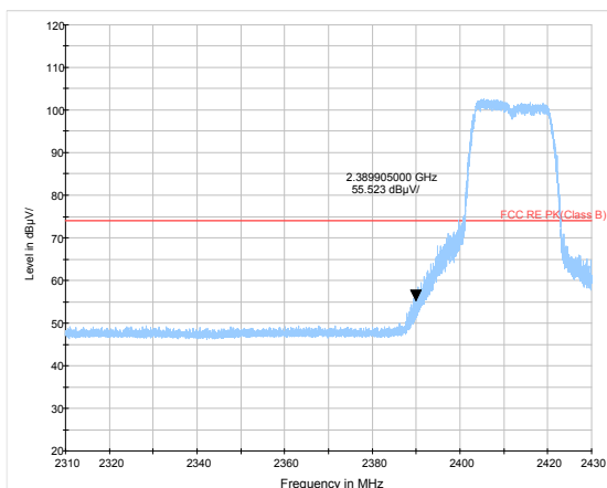
802.11n HT20 -Channel 1 Peak
