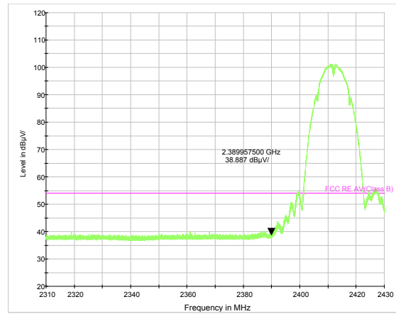
802.11b-Channel 1 Average
