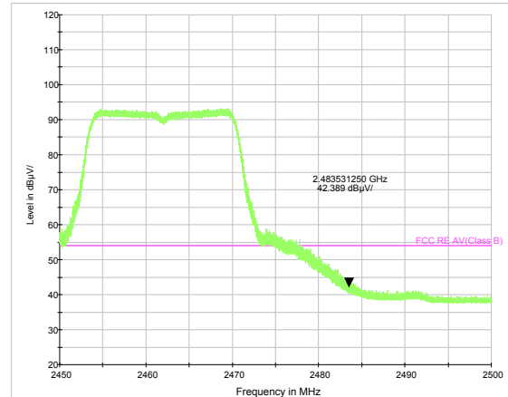
802.11g-Channel 11 Average
