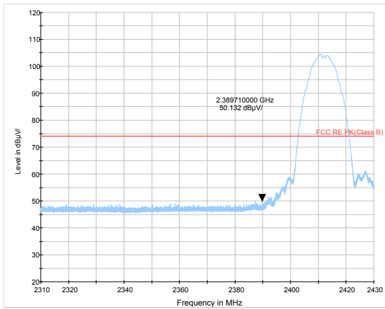
802.11b-Channel 1 Peak
