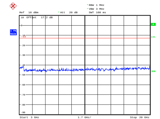
GSM 1900 CH-Low 3GHz~20GHz
