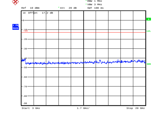
GSM 1900 CH-Middle 3GHz~20GHz
