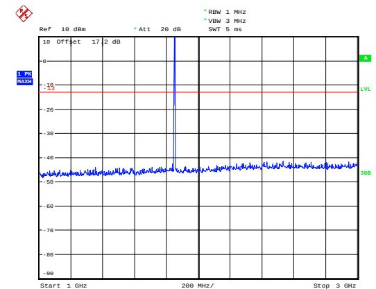
GSM 1900 CH-Low 1GHz~3GHz
