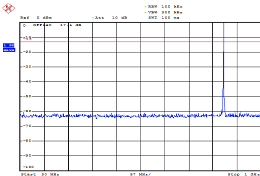
GSM 850 CH-High 30MHz ~ 1GHz
