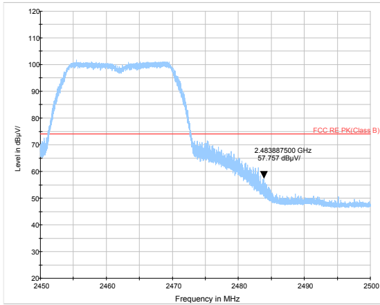
802.11g-Channel 11 Peak
