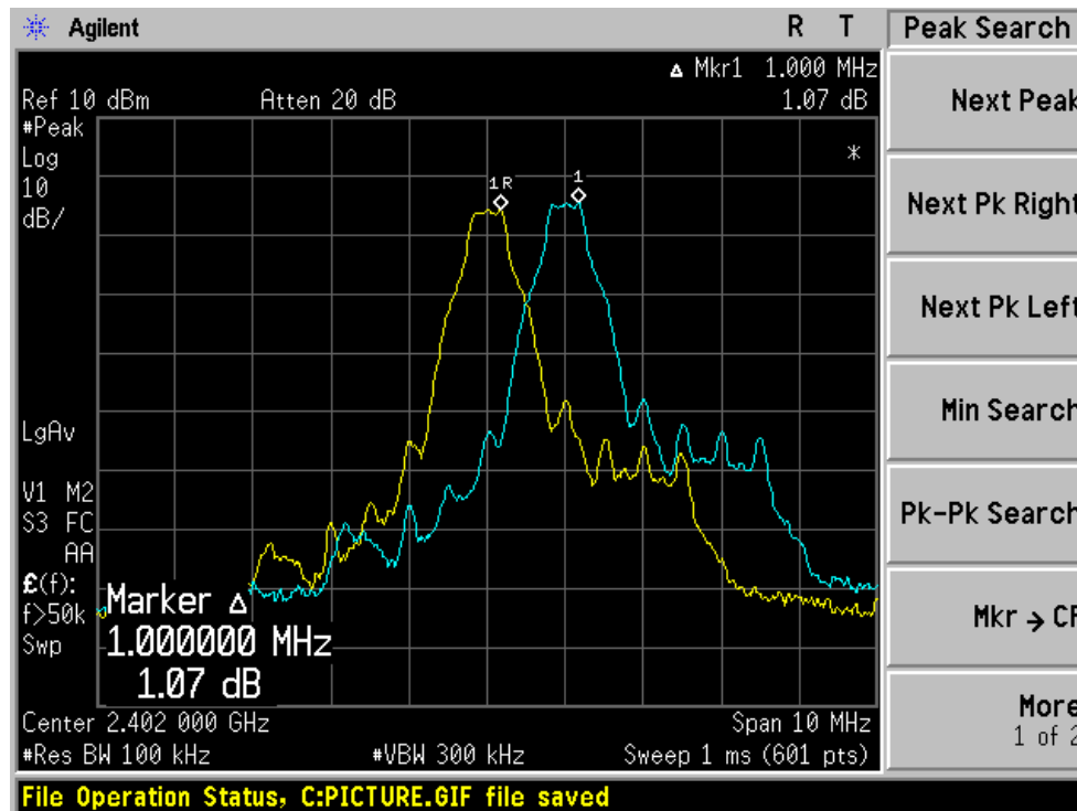
Channel 00 (2402MHz)
