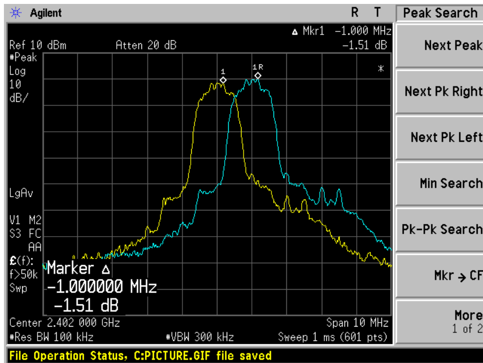
Channel 00 (2402MHz)
