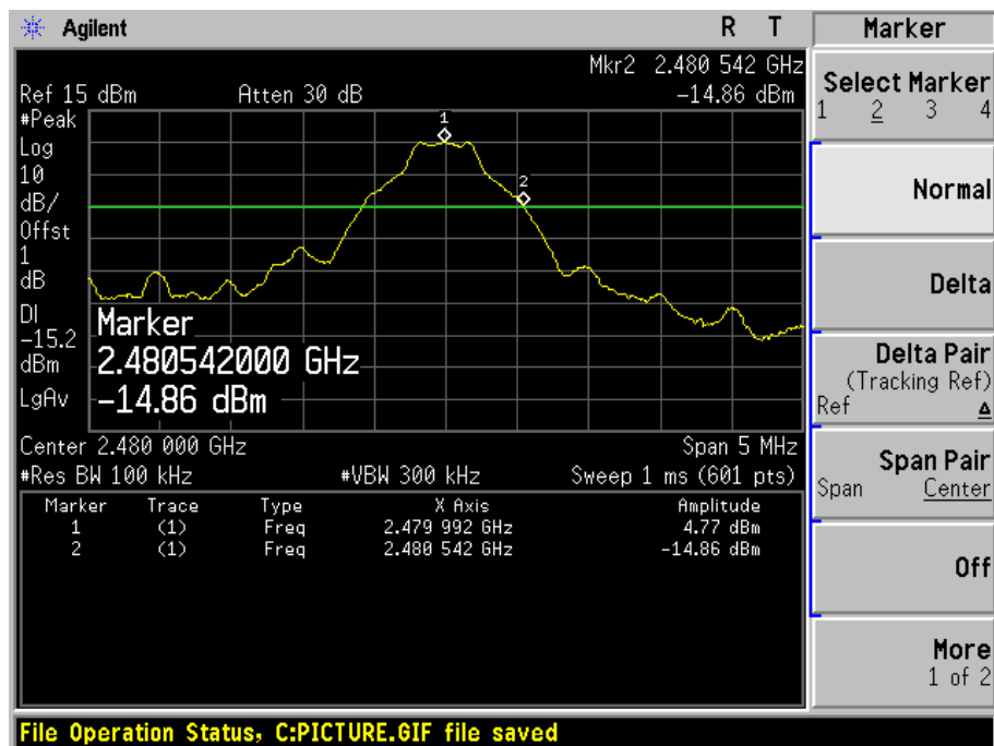
Channel 78 (2480MHz)
