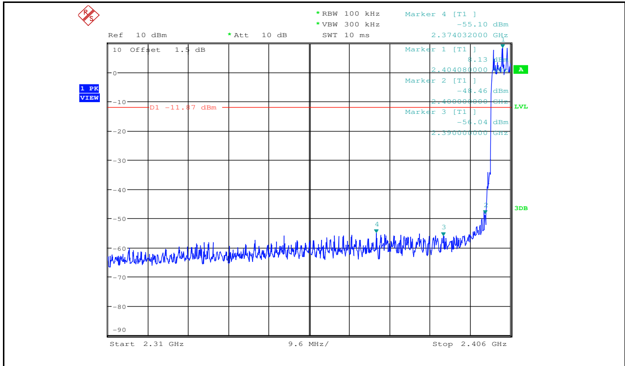
Band-edge for RF Conducted Emissions_2DH5_2402_Hopping Off
