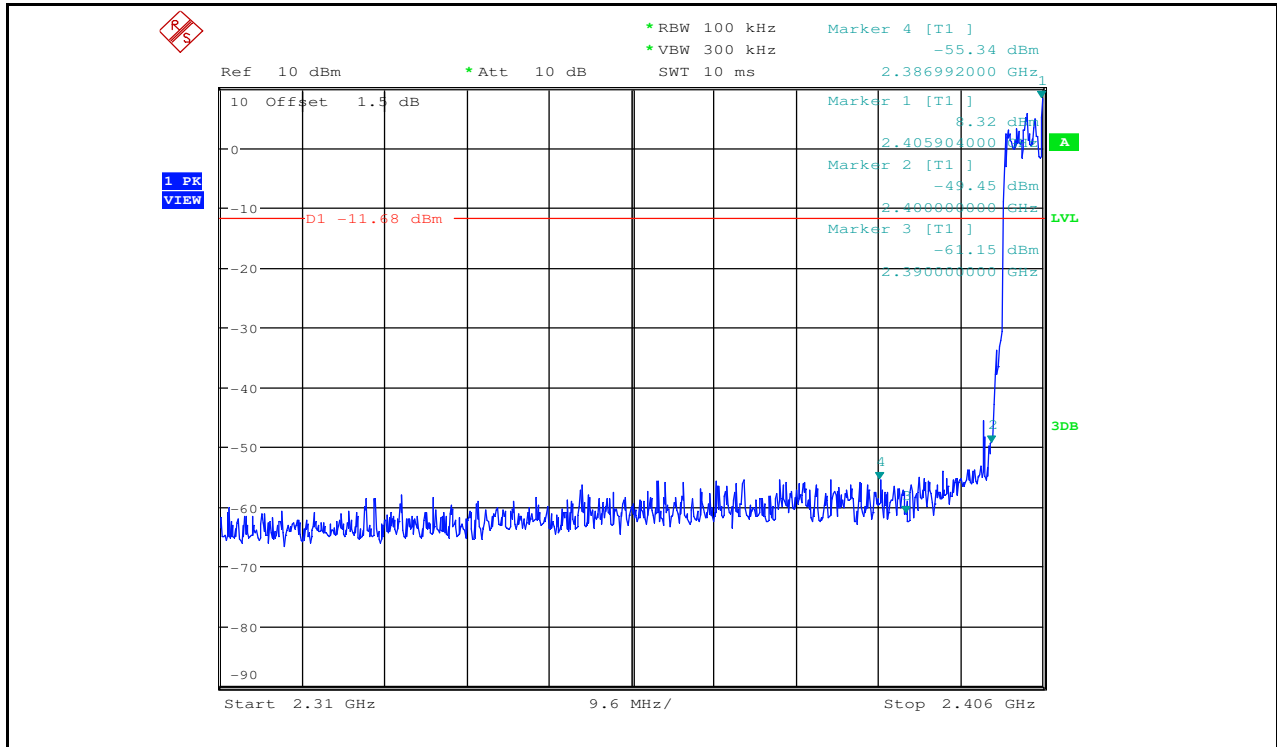
Band-edge for RF Conducted Emissions_3DH5_2402_Hopping Off
