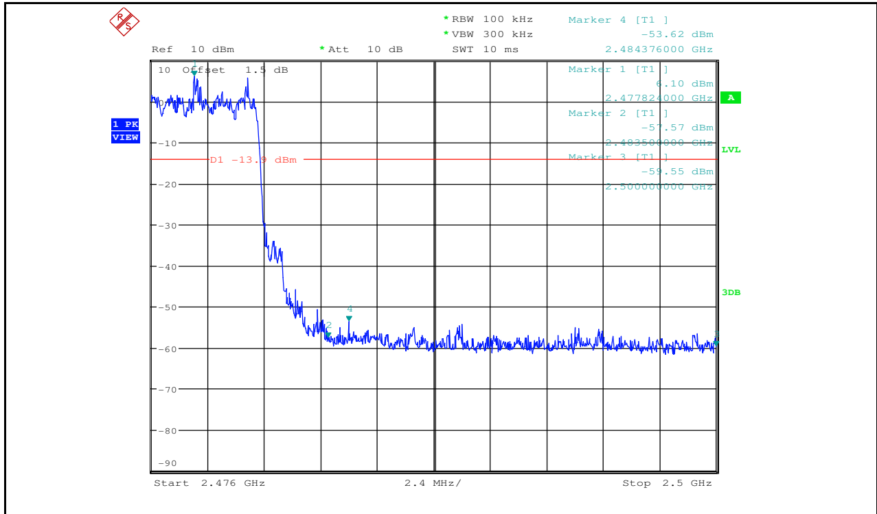
Band-edge for RF Conducted Emissions_2DH5_2480_Hopping Off
