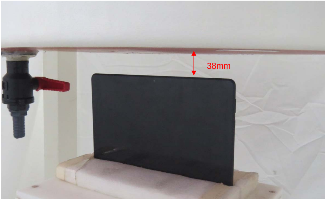
Picture 5: Top Side, the distance from handset to the bottom of the Phantom is 38mm
