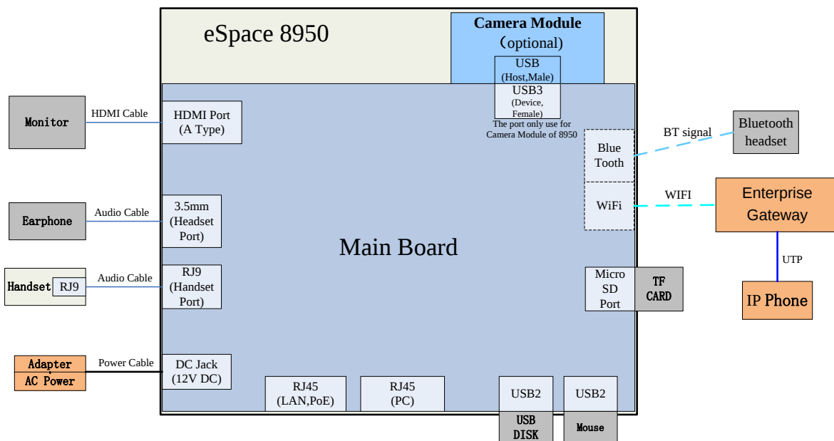
Figure 16. Test connection of TC3
