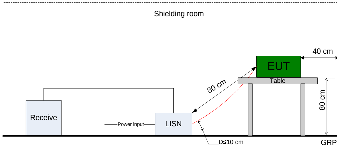
Figure 19. Test set-up of conducted disturbance for power port
