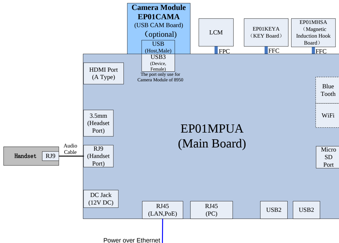
Figure 13. Test Configuration 2 (TC2)
