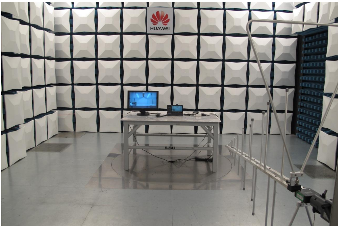
Radiated emission for 30 MHz to 1 GHz
