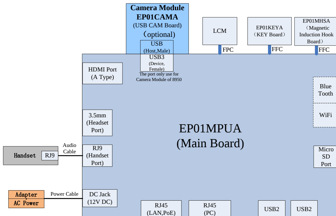
Figure 12. Test Configuration 1 & 3 (TC1 & TC3)
