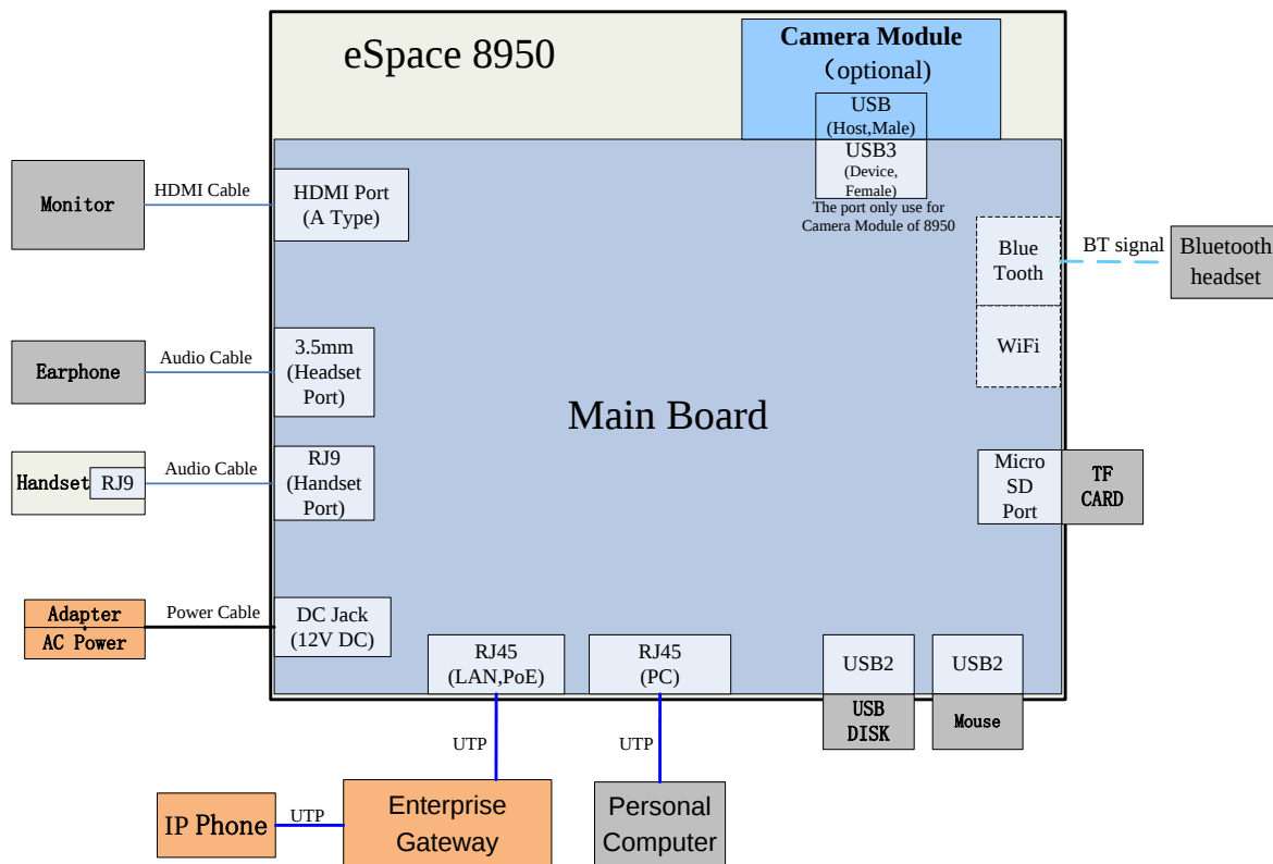
Figure 14. Test connection of TC1
