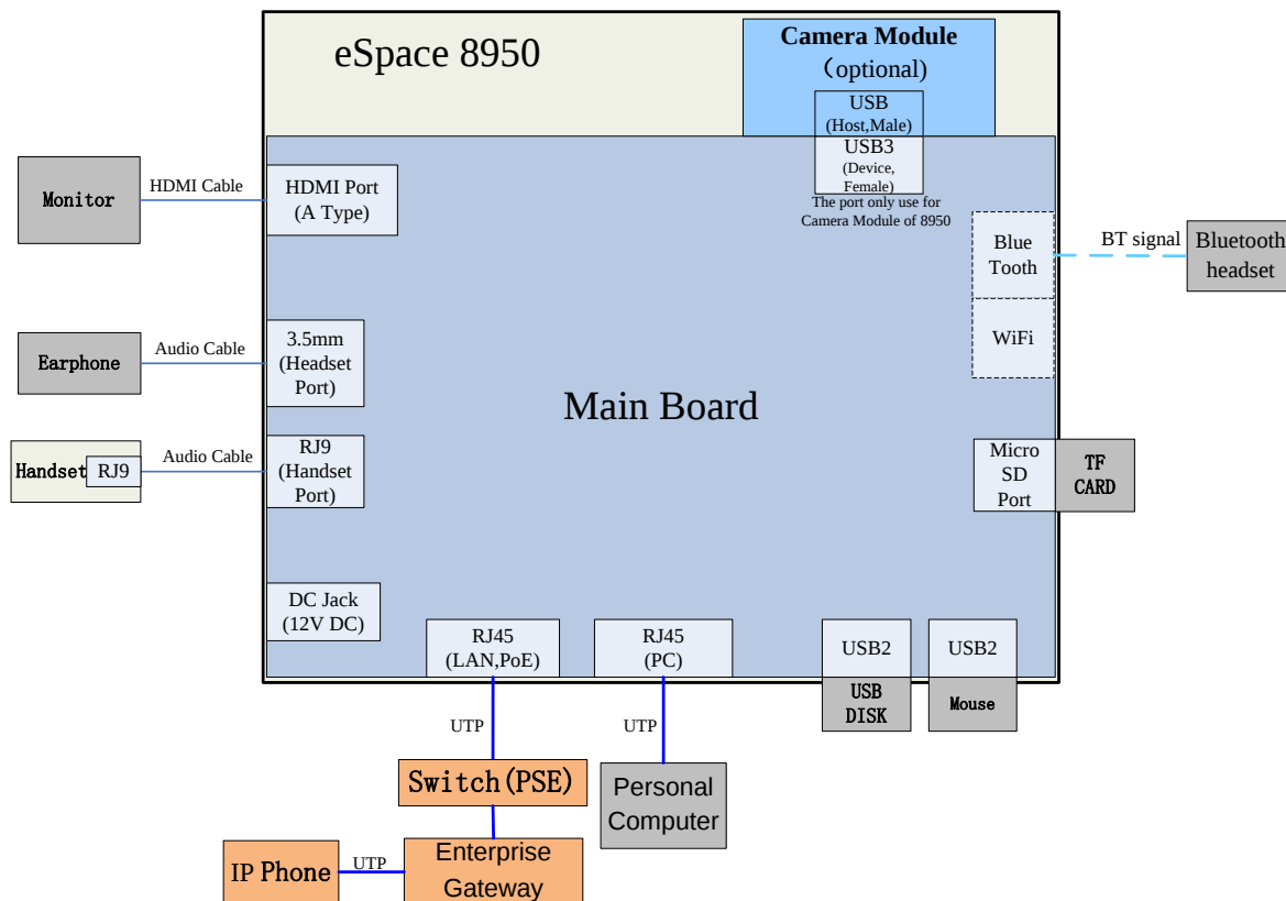
Figure 15. Test connection of TC2
