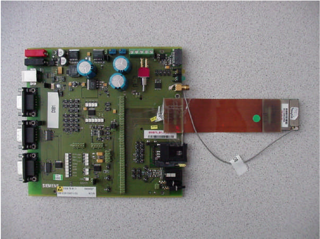
Photo 5: DSB75 Evaluation Board (without housing), Flex Cable, EUT
