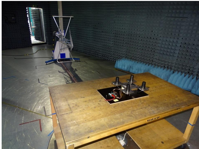
Photo 1: Test setup for radiated measurements below 1 GHz
