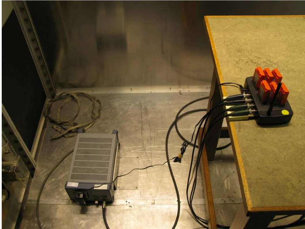
Photograph 4: - AW-A Wireless base station, test setup conducted emissions on AC mains
