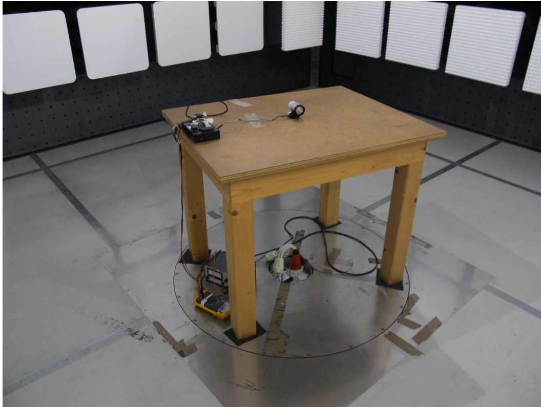
Photograph 2: - EUT on radiated emissions test table
