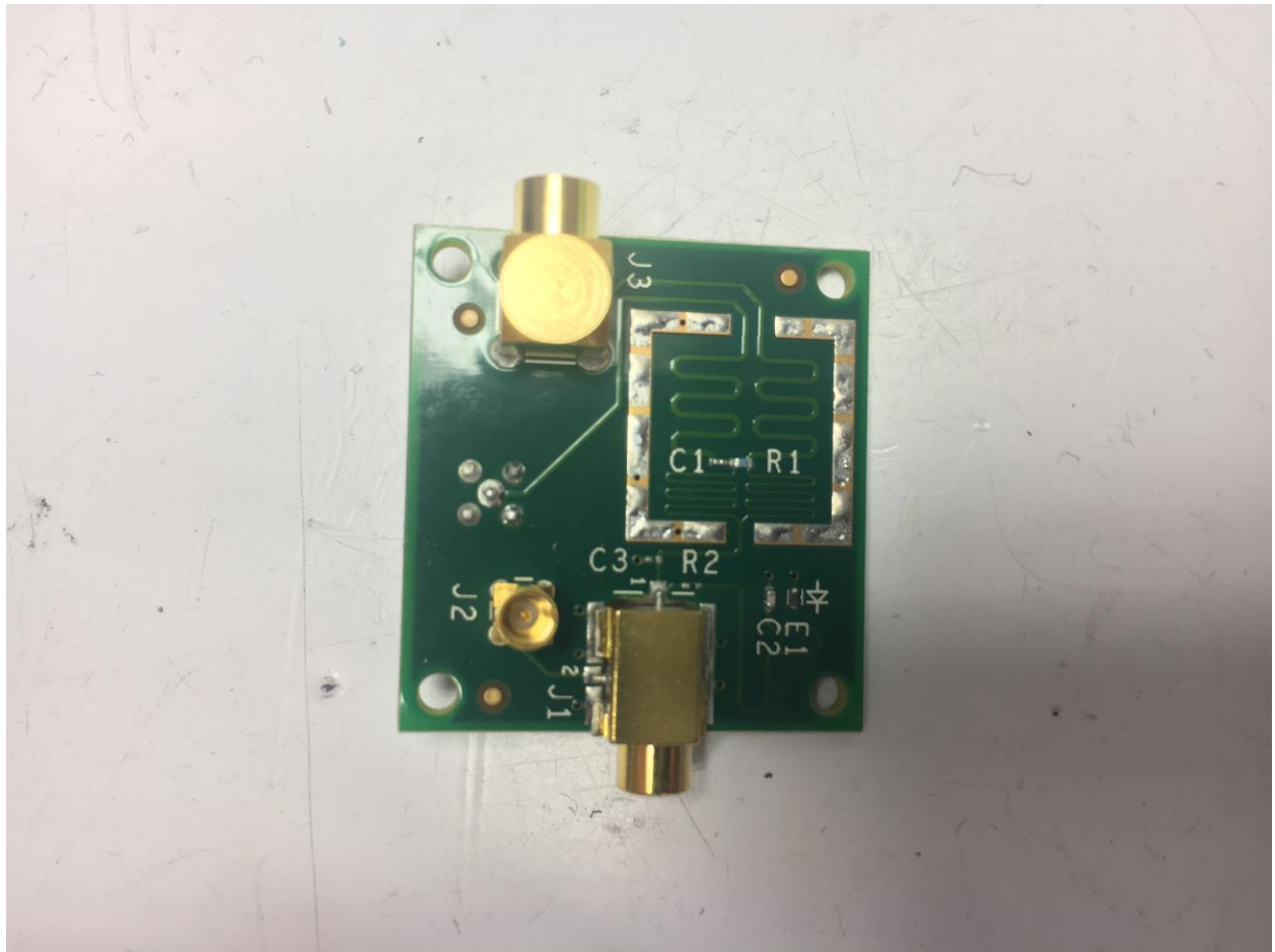
Photograph 7. Board 3
