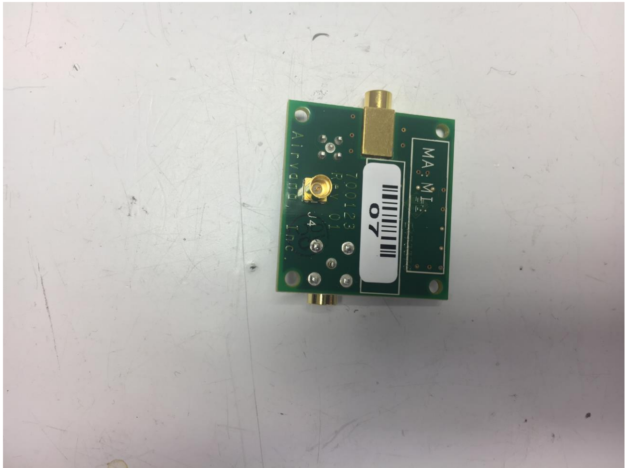
Photograph 8. Board 3 back
