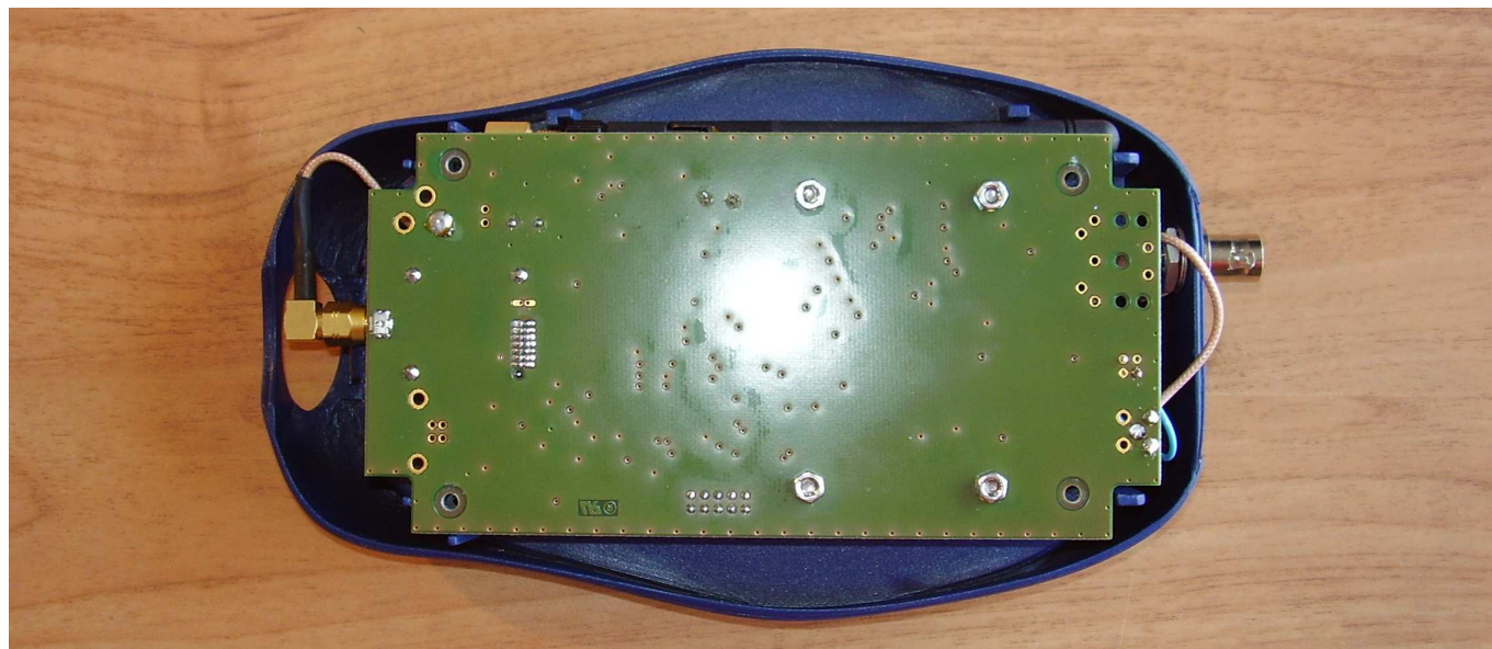
Reader (without rear plastic cover)
