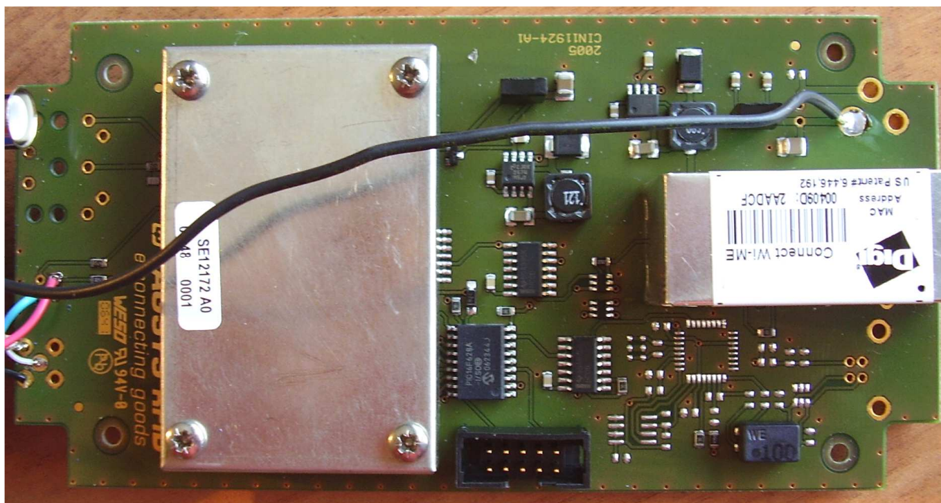
PCB (Reader)
