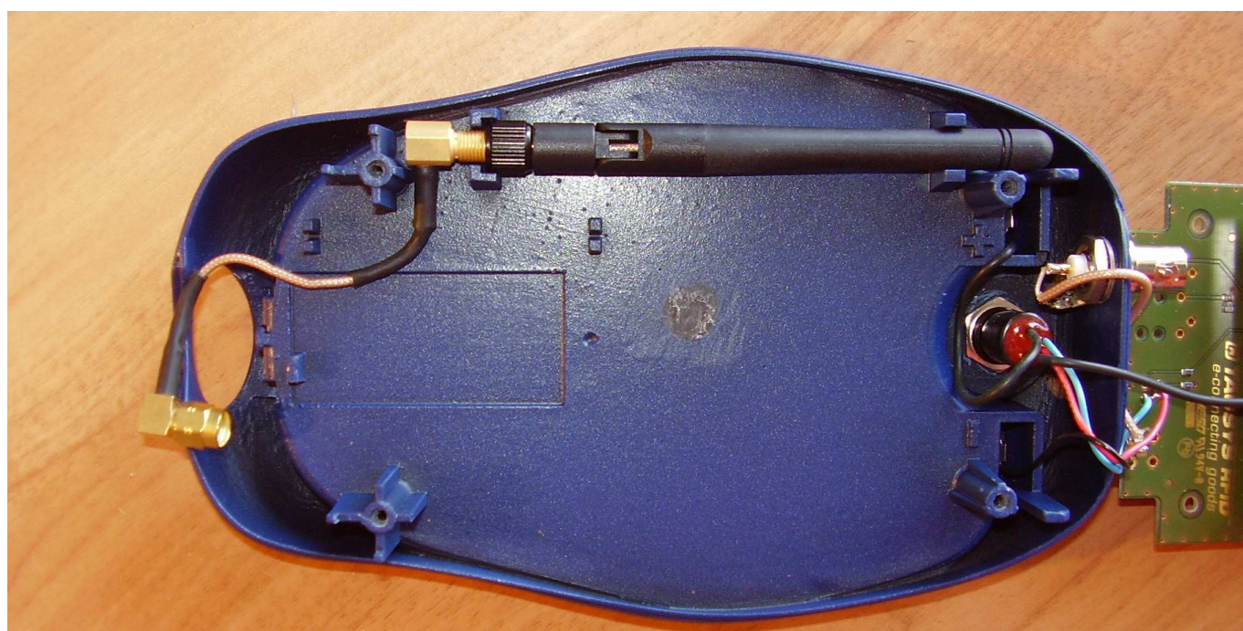
Reader (PCB removed)
