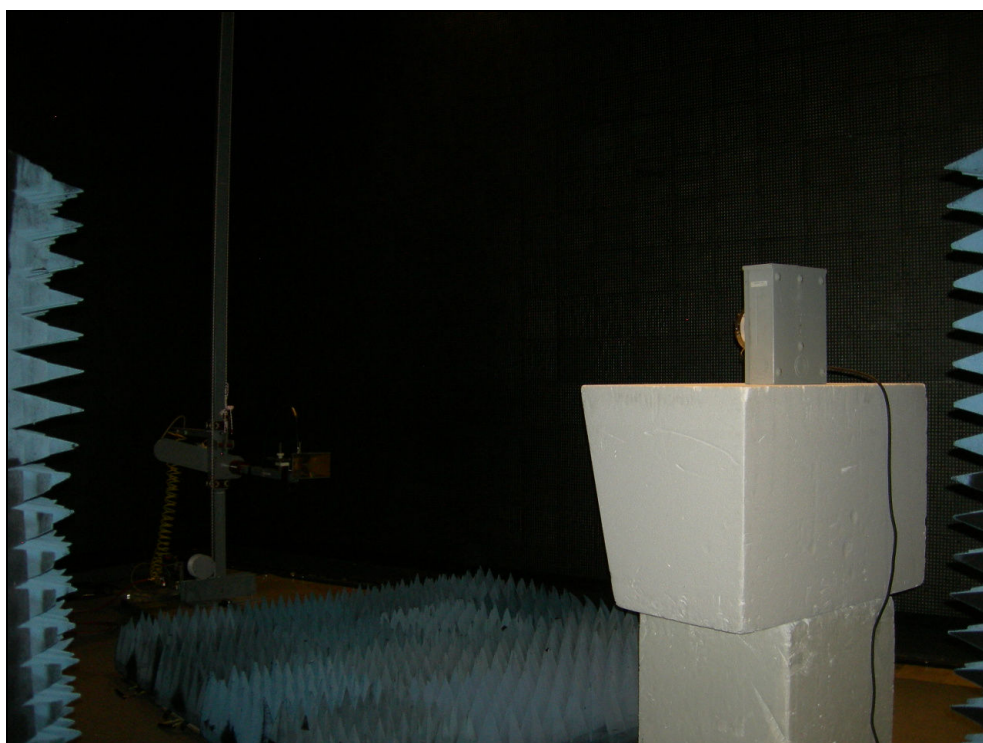
Figure 12: Collocated/Simultaneous Transmission Test Setup (Meter)
