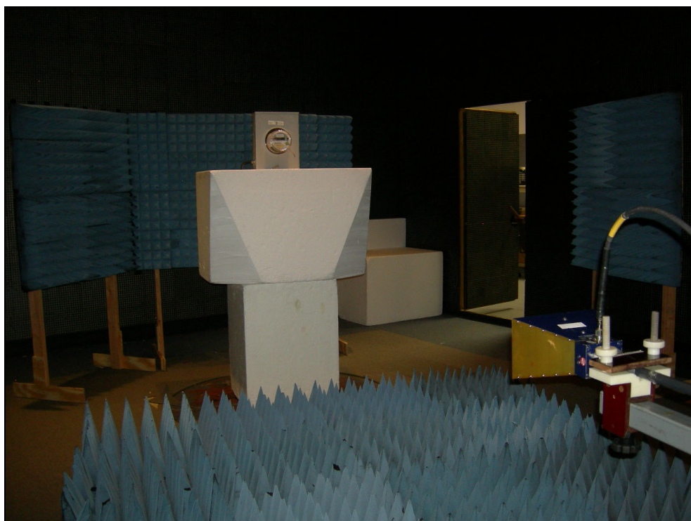
Figure 13: Collocated/Simultaneous Transmission Test Setup (Meter)
