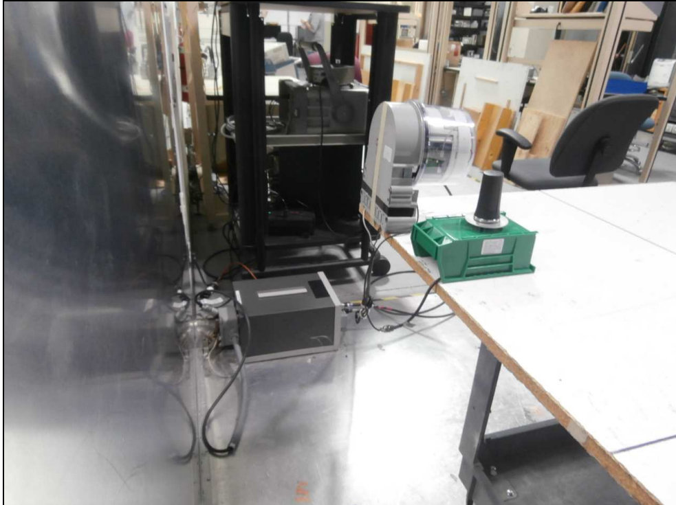
Figure 26: Conducted Emissions – 9S Meter Form
