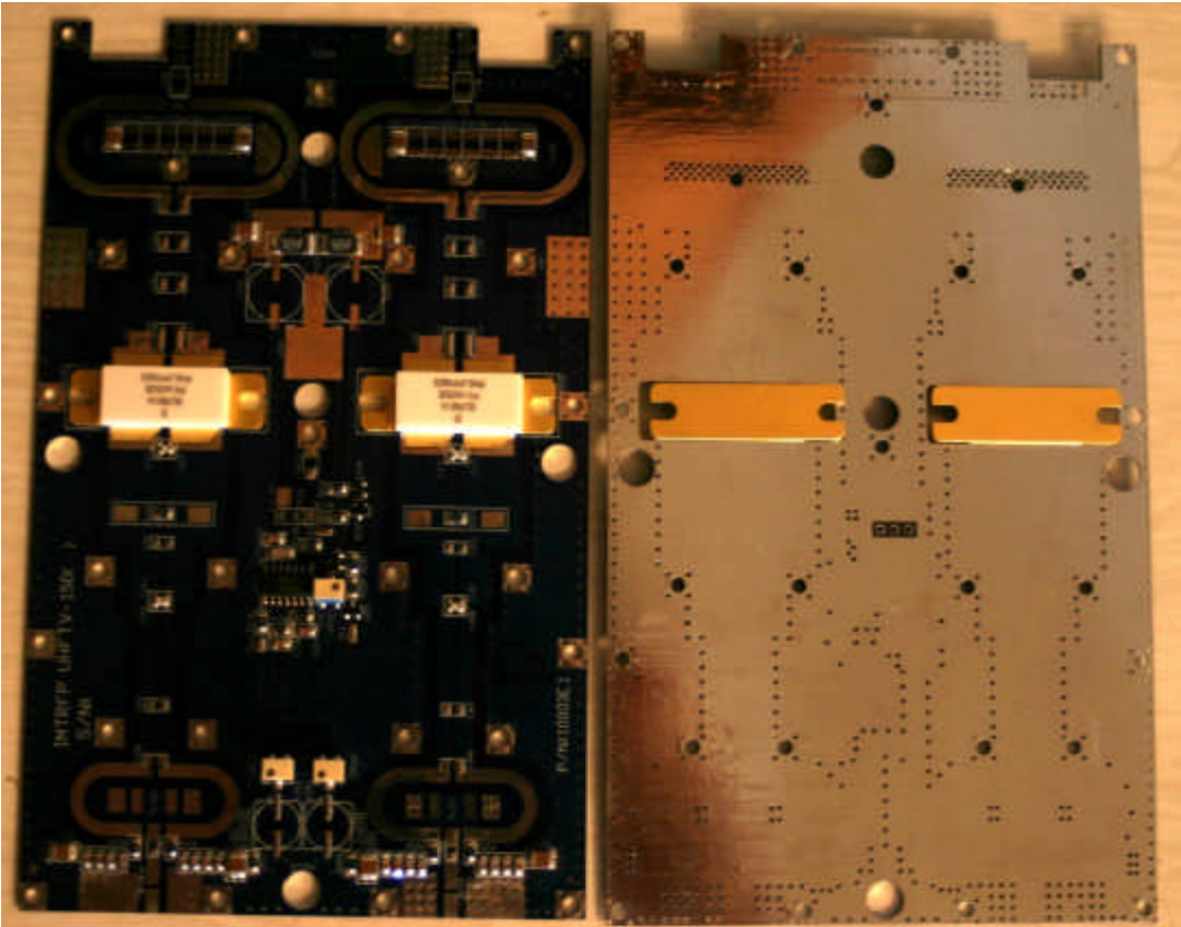
UHFTV-150 (bottom and top side with all devices populated):
