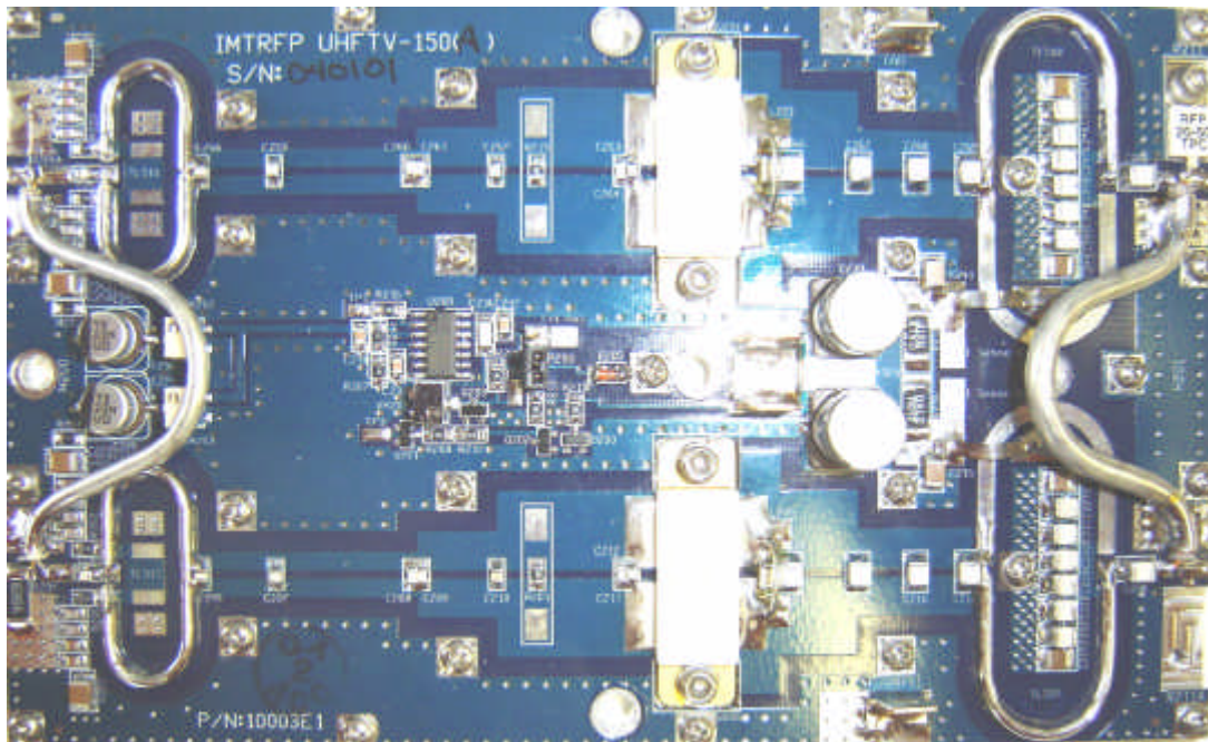
UHFTV-150 (top side):
