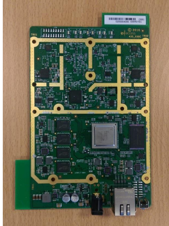
Heatsink removed
