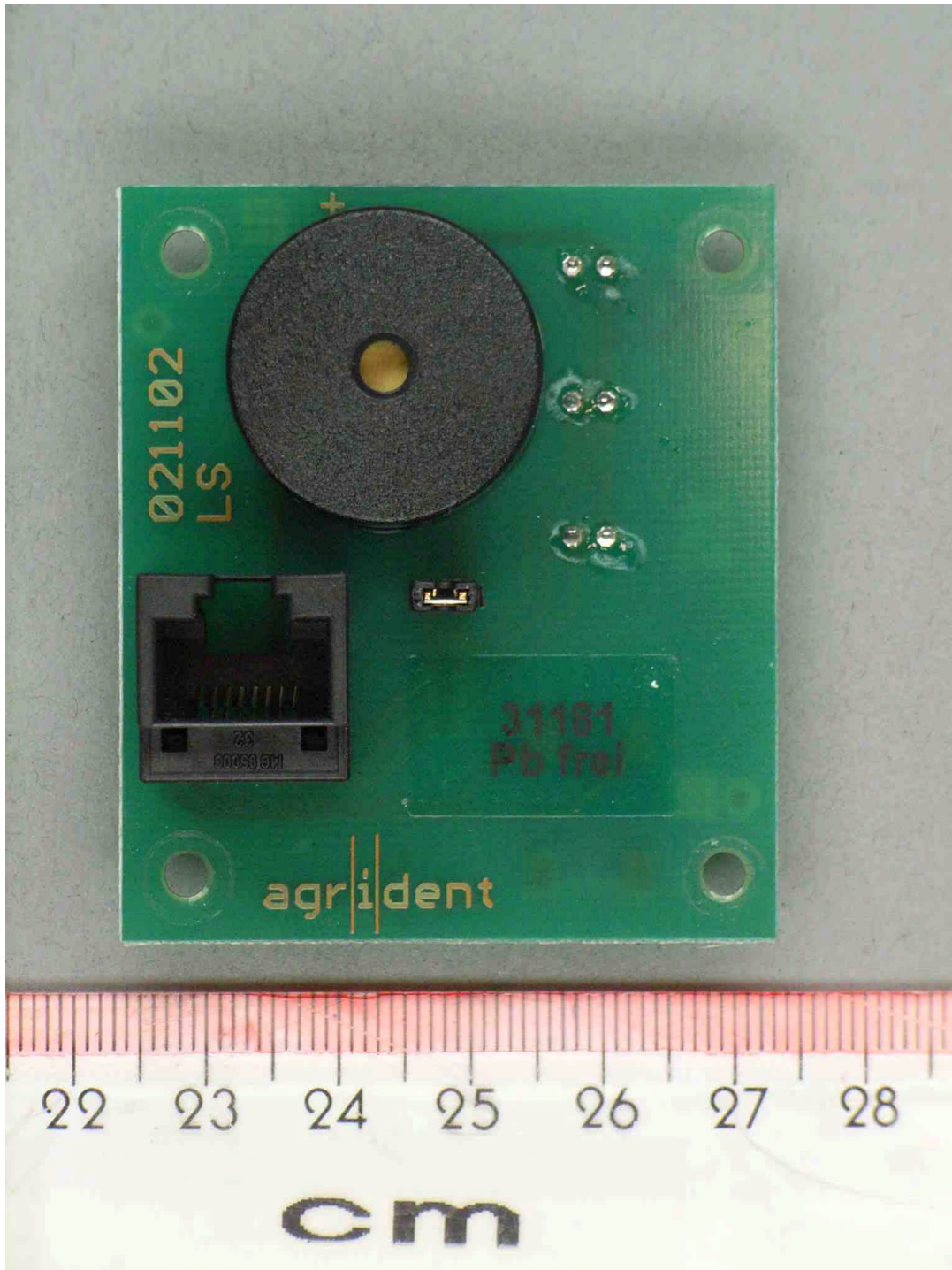
70543_10.jpg ASR700, panel PCB, top view
