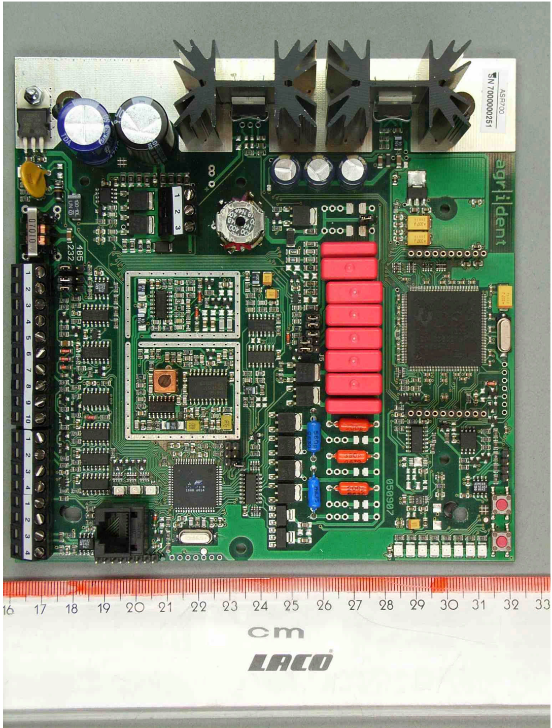
70543_12.jpg ASR700, PCB, top view
