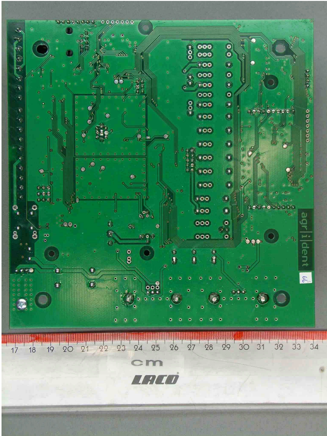
70543_11.jpg ASR700, PCB, bottom view
