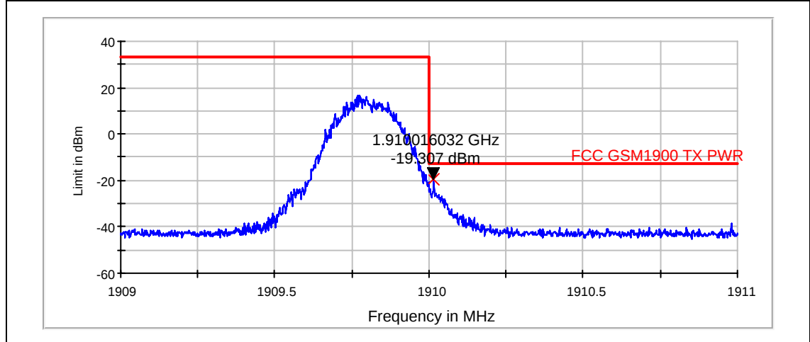
EGPRS, channel 810 / 1909.8 MHz (Peak detector, RBW: 3 kHz)
