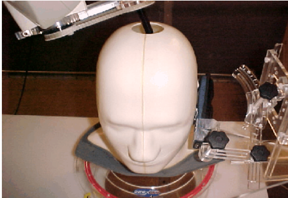
Figure S7. Configuration #7 - Cheek (0°) position, right side, GPS In, 900 mAH Battery
