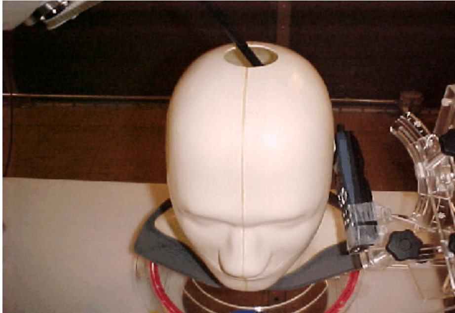
Figure S5. Configuration #5 - Tilt (15°) position, right side, GPS In, 900 mAH Battery
