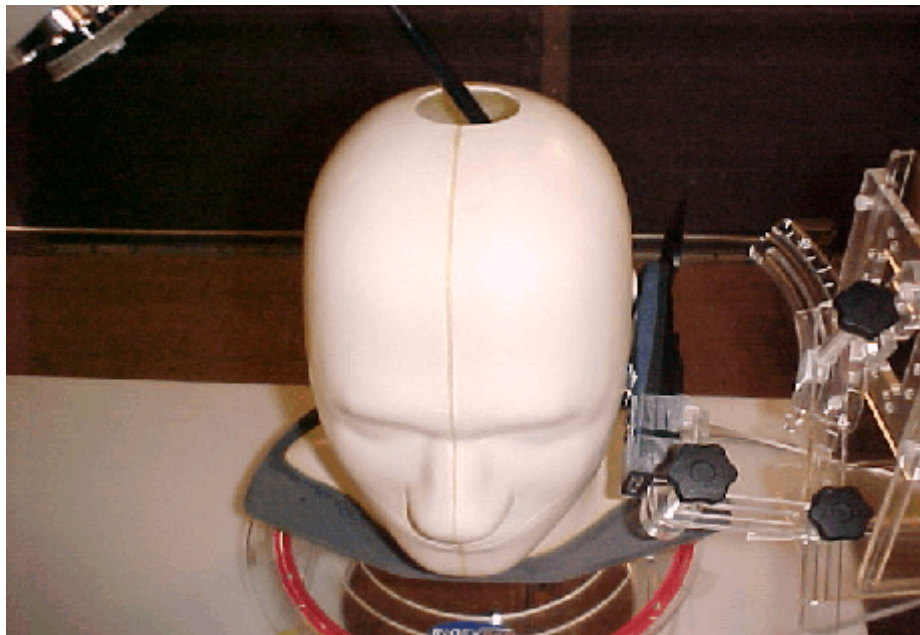
Figure S8. Configuration #8 - Cheek (0°) position, right side, GPS Out, 900 mAH Battery
