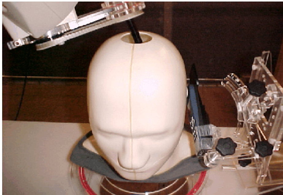
Figure S6. Configuration #6 - Tilt (15°) position, right side, GPS Out, 900 mAH Battery
