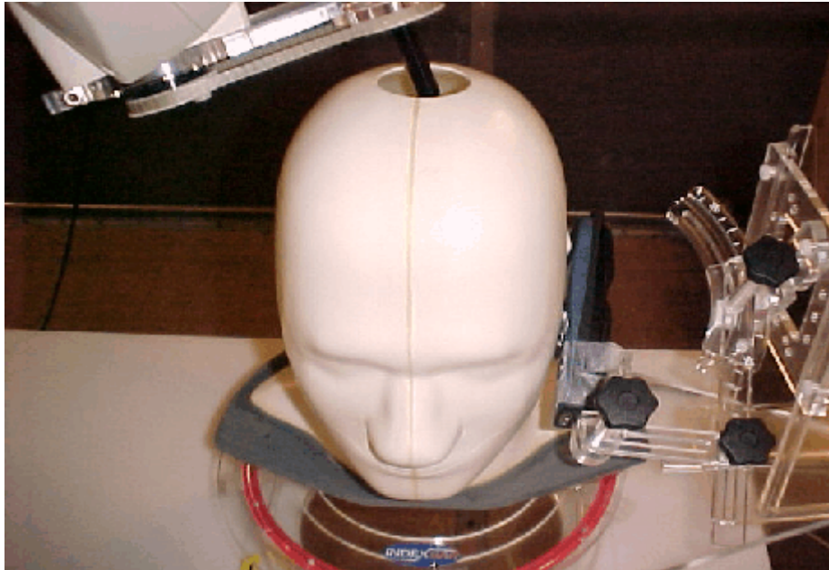
FigureS3. Configuration #3 - Cheek ( 0^{\circ} ) position, right side, GPS In, 1200 mAH Battery
