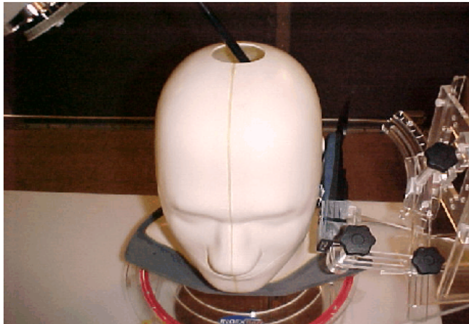
Figure S4. Configuration #4 - Cheek ( 0^{\circ} ) position, right side, GPS Out, 1200 mAH Battery
