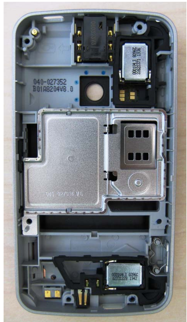
Fig 6 – Back Housing
