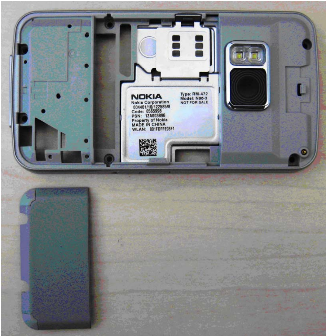
Fig 9 – Rear Housing with Antenna module removed
