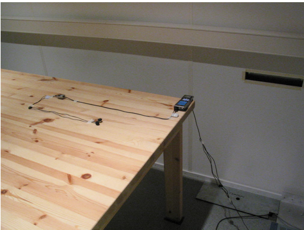
Picture 4 AC powerline conducted emission measurement (GSM1900, BlueTooth)
