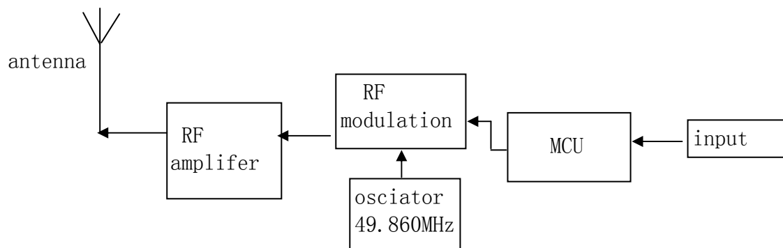
45070 49m tx circuit block diagram
