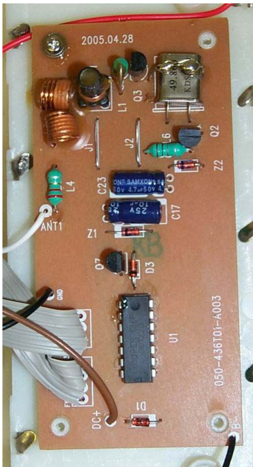
Component Side
