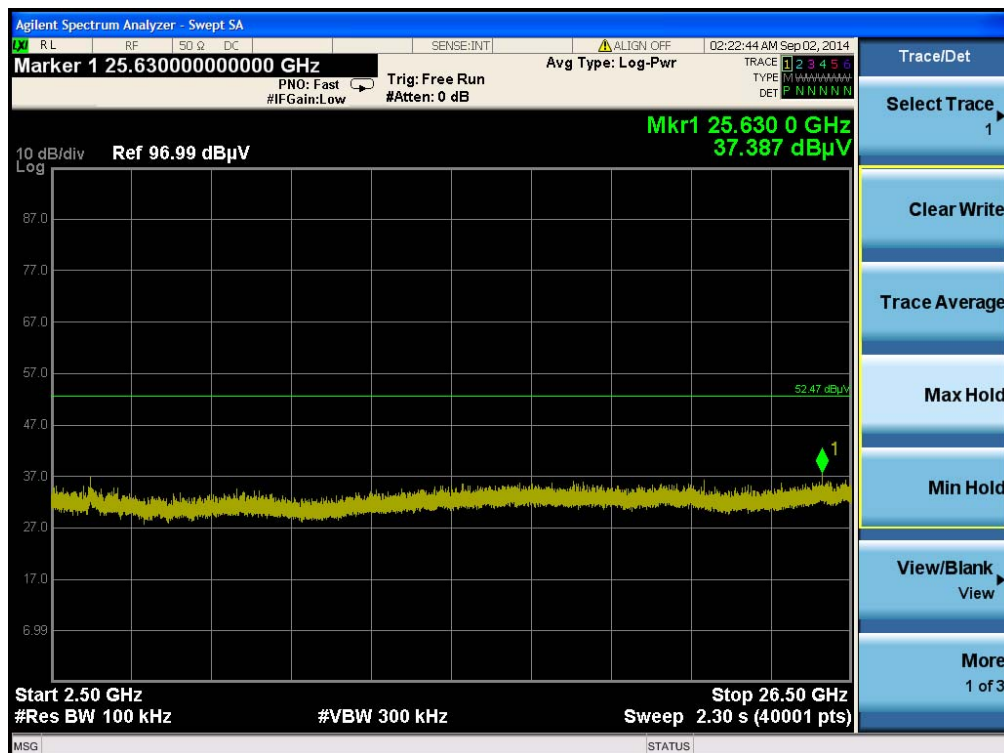
Plot on Configuration For BR (GFSK) / Hopping / 2500MHz~26500MHz (down 30dBc) (Vertical)
