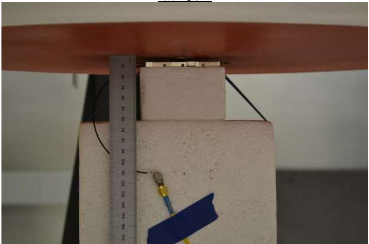
Bottom @ 5mm
