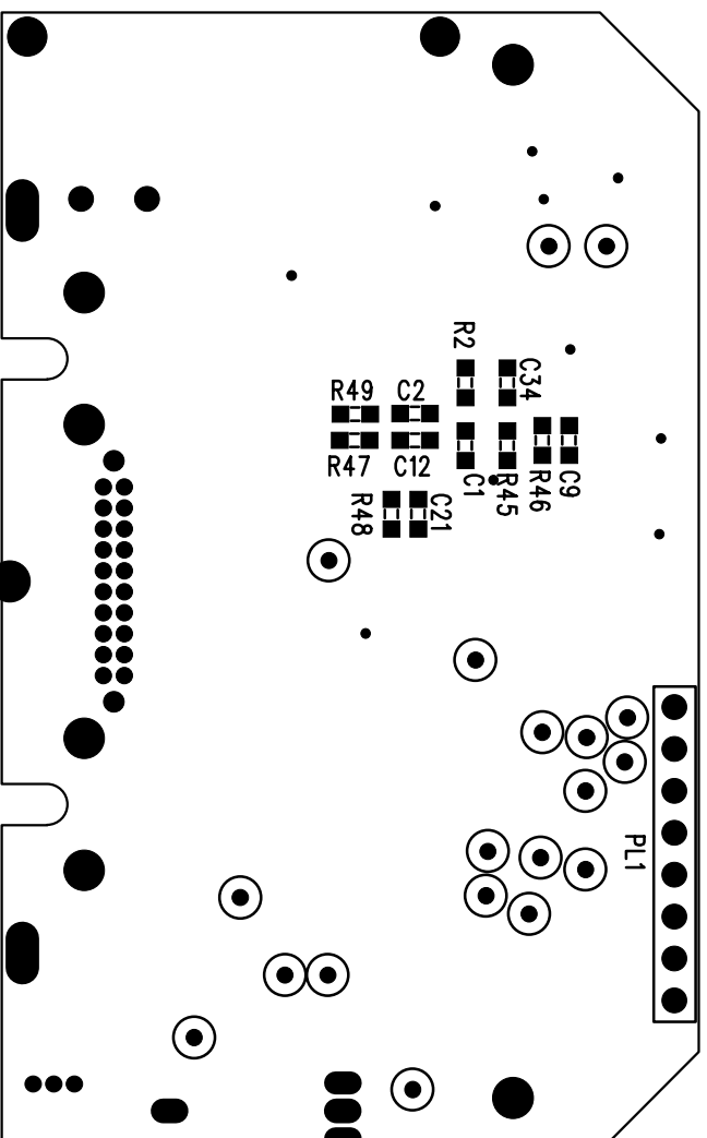
ANNOTATION ISS 1 – TRACK A Q-Bot Interface MK 2
