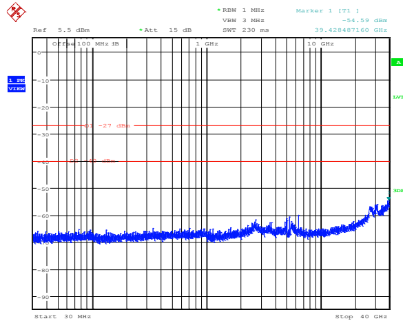
Diagram 8.5-19: Conducted spurious emissions for FCC, 10 dBi antenna, 20 MHz channel, cho, mid frequency
