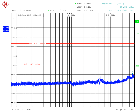
Diagram 8.5-31: Conducted spurious emissions for FCC, 19 dBi antenna, 10 MHz channel, cho, mid frequency
