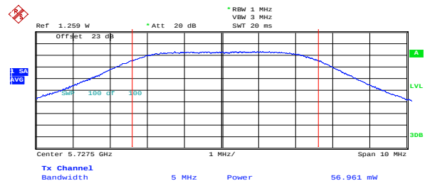
Antenna Port 2
