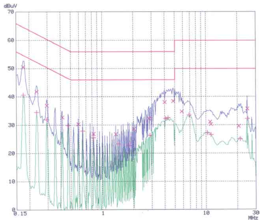
< Neutral line >
