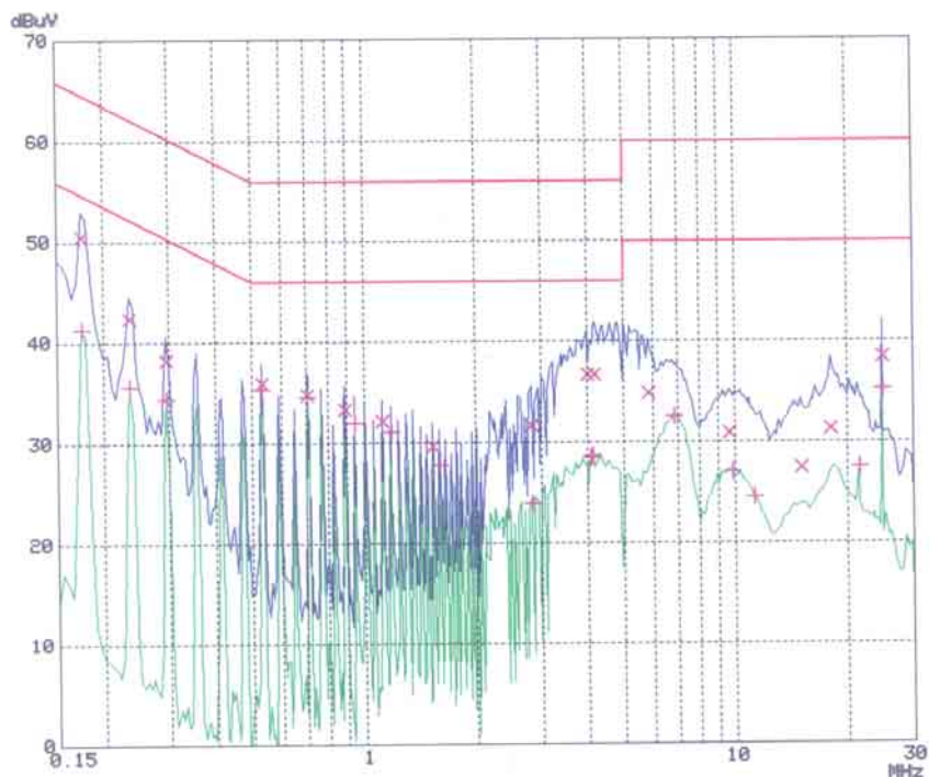
< Hot line >
