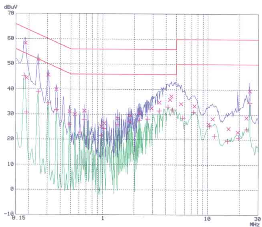
< Neutral line >
