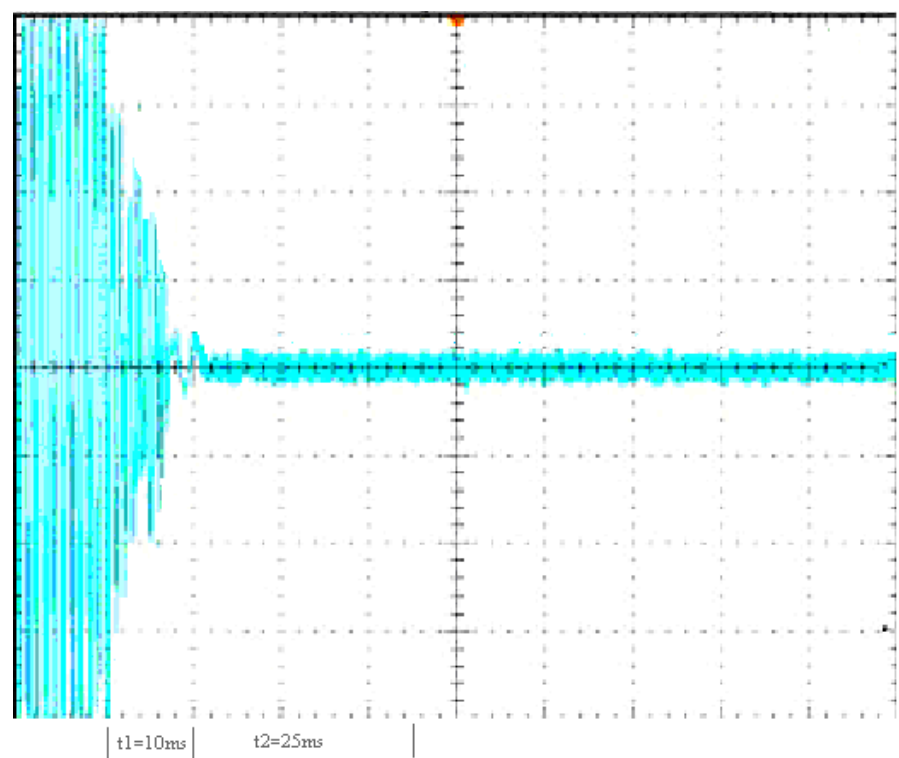
Transmitter Frequency Behaviour @ 25 KHz Channel Separation--On to Off
