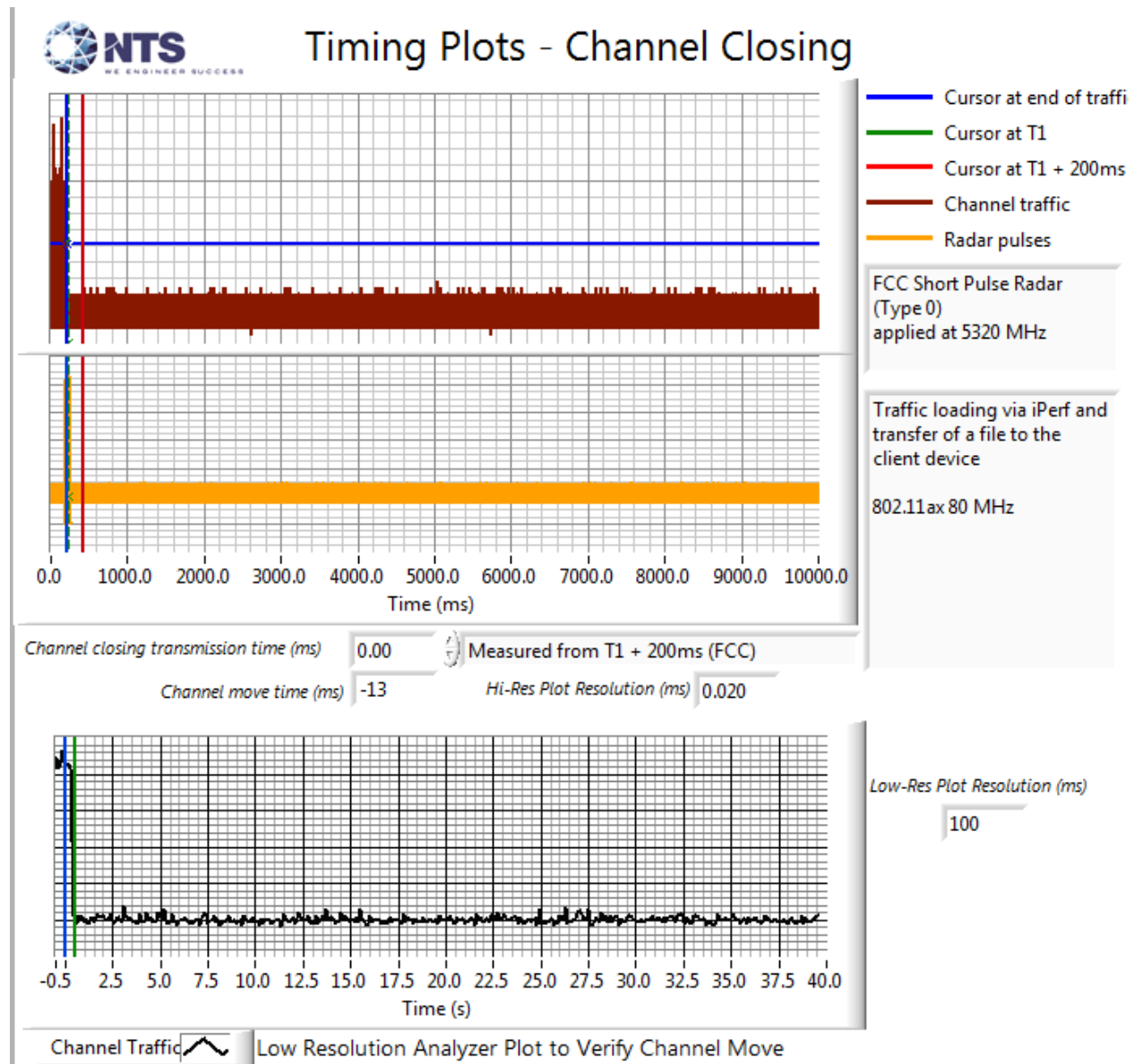
Figure 21 Channel Closing &amp; Channel Move Time (Tri Radio 80MHz Low Band) plot
