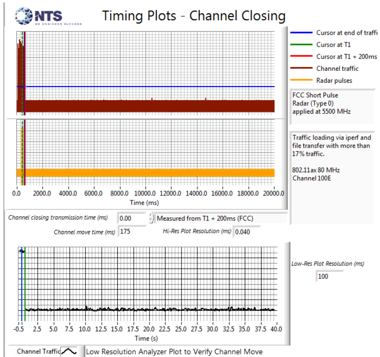
Figure 23 Channel Closing &amp; Channel Move Time (Tri Radio 80MHz High Band) plot
