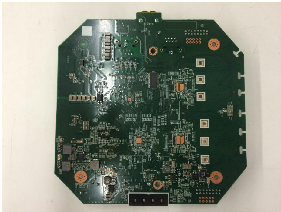
BACK SIDE OF PCB WITHOUT SHIELDS
