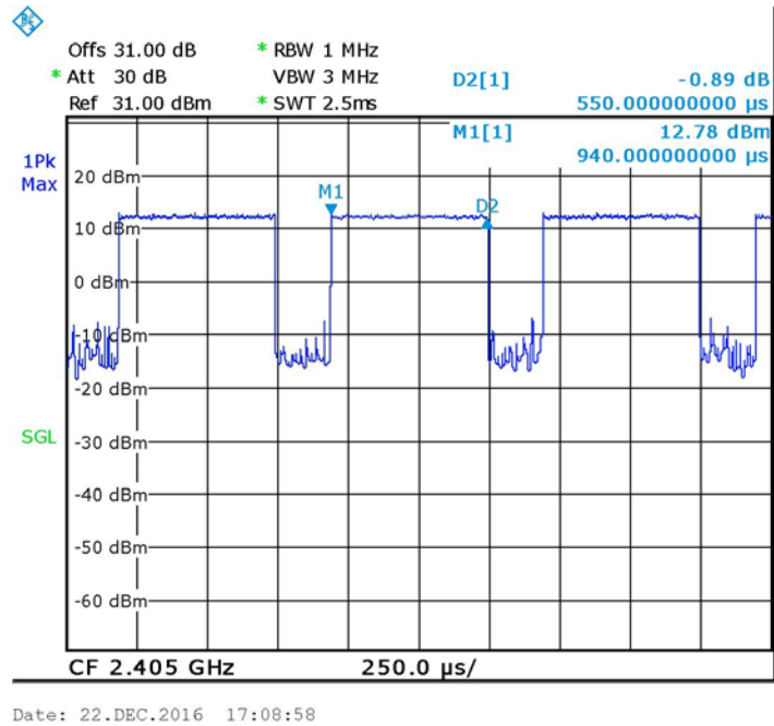
Figure 40. Burst Duration
