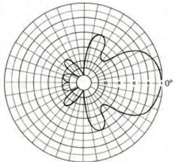
VERTICAL POLARIZATION
