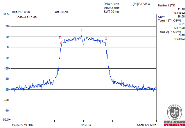
802.11ac (VHT40)_Chain 3 / CH38
