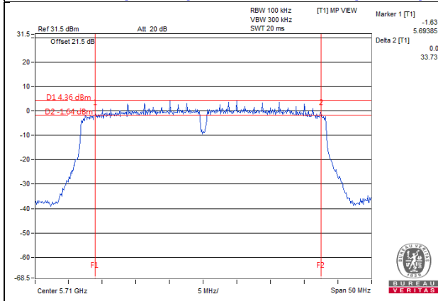
802.11ac (VHT40)_Chain 3 / CH142 (U-NII-3)
