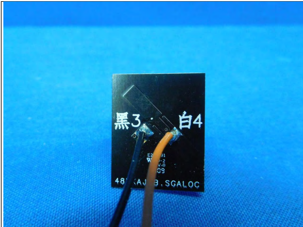
2.4G Ant 2 / 5G HB Ant 4
