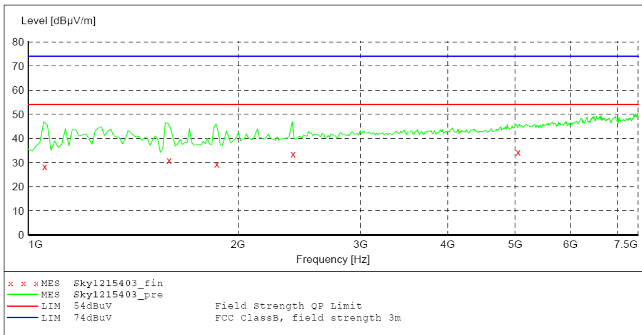
(Plot C: Test Antenna Horizontal 1G – 7.5G)
