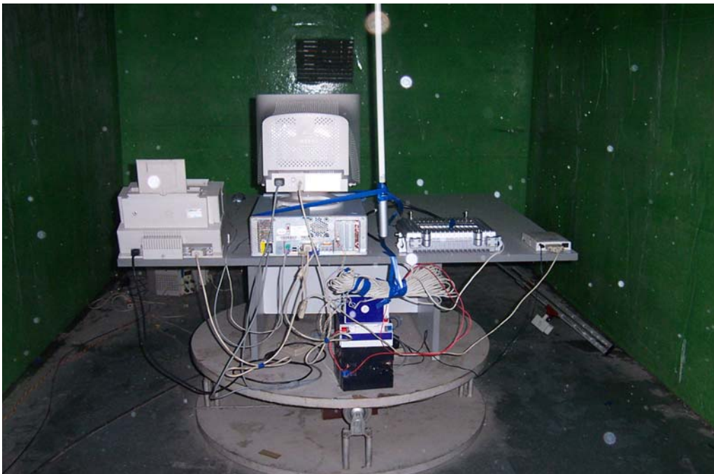
Antenna TQJ-2.4G-8: Radiated Emission - Rear View
