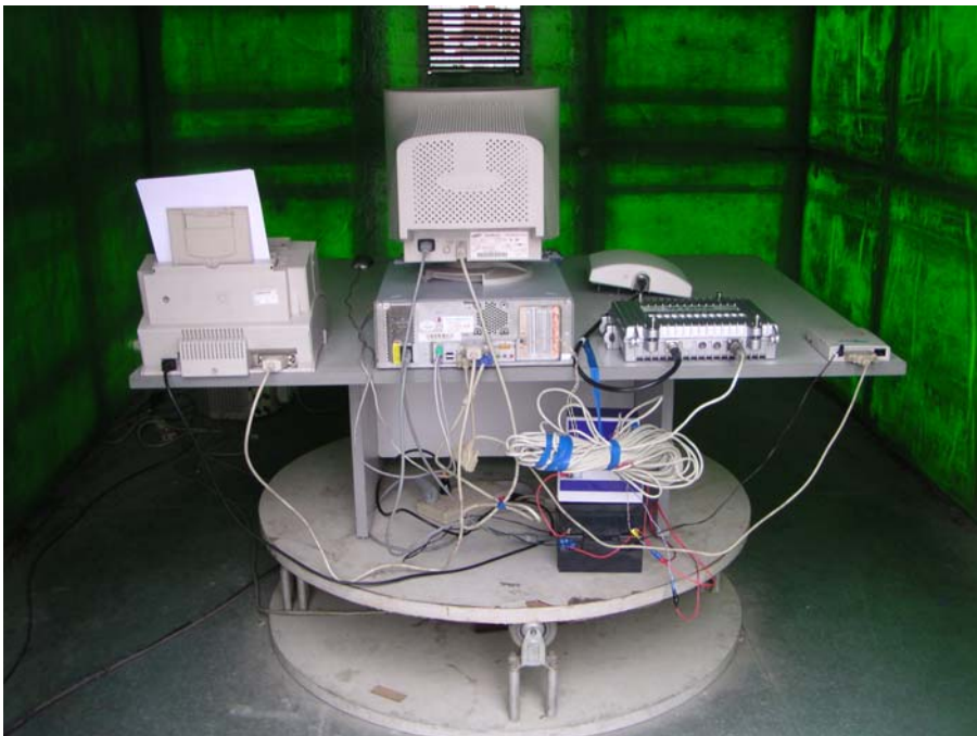
Antenna MB2400-30-14: Radiated Emission - Rear View
