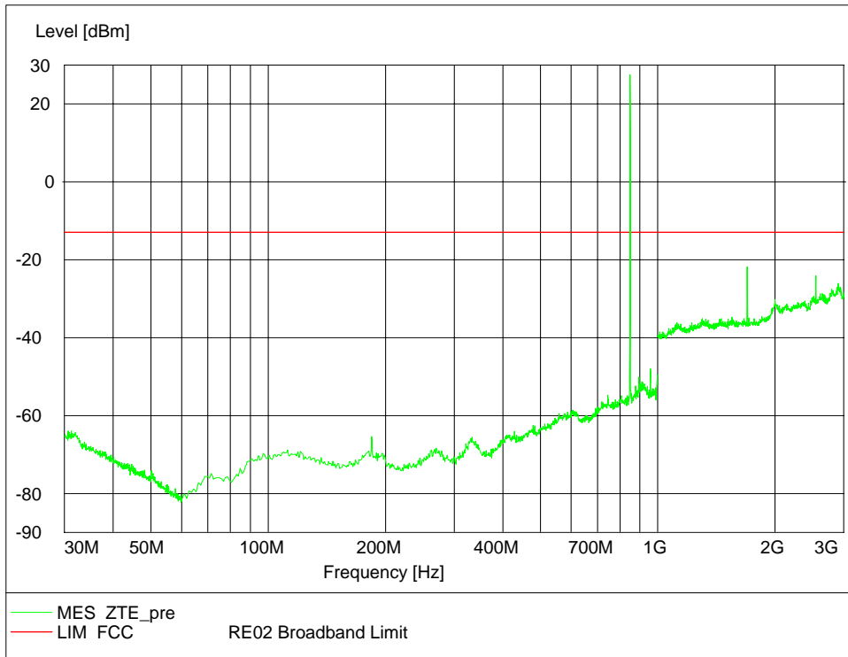
Channel 189, 30MHz~3GHz
