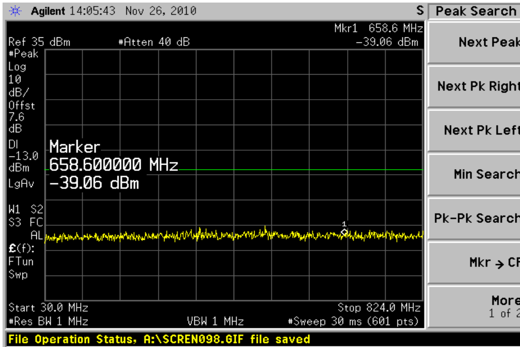
Channel 189, 30MHz~824MHz
