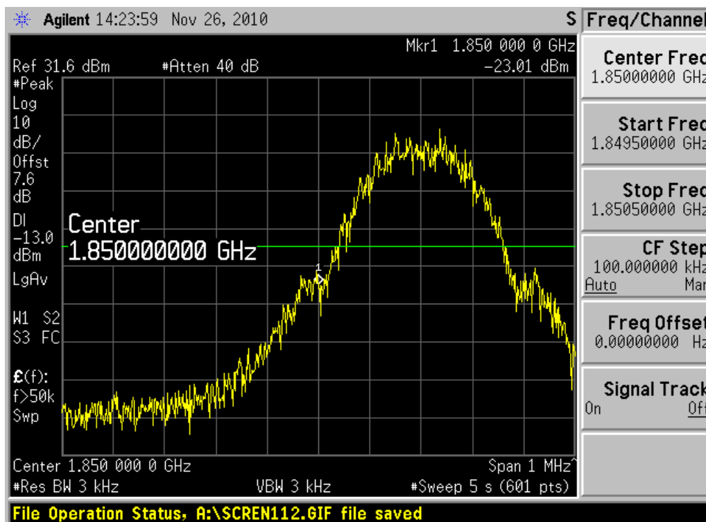
Channel 512
