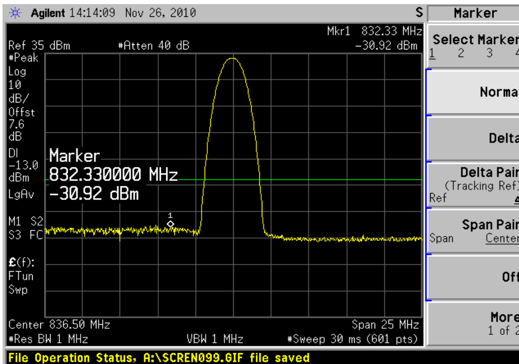
Channel 189, 824MHz~849MHz
