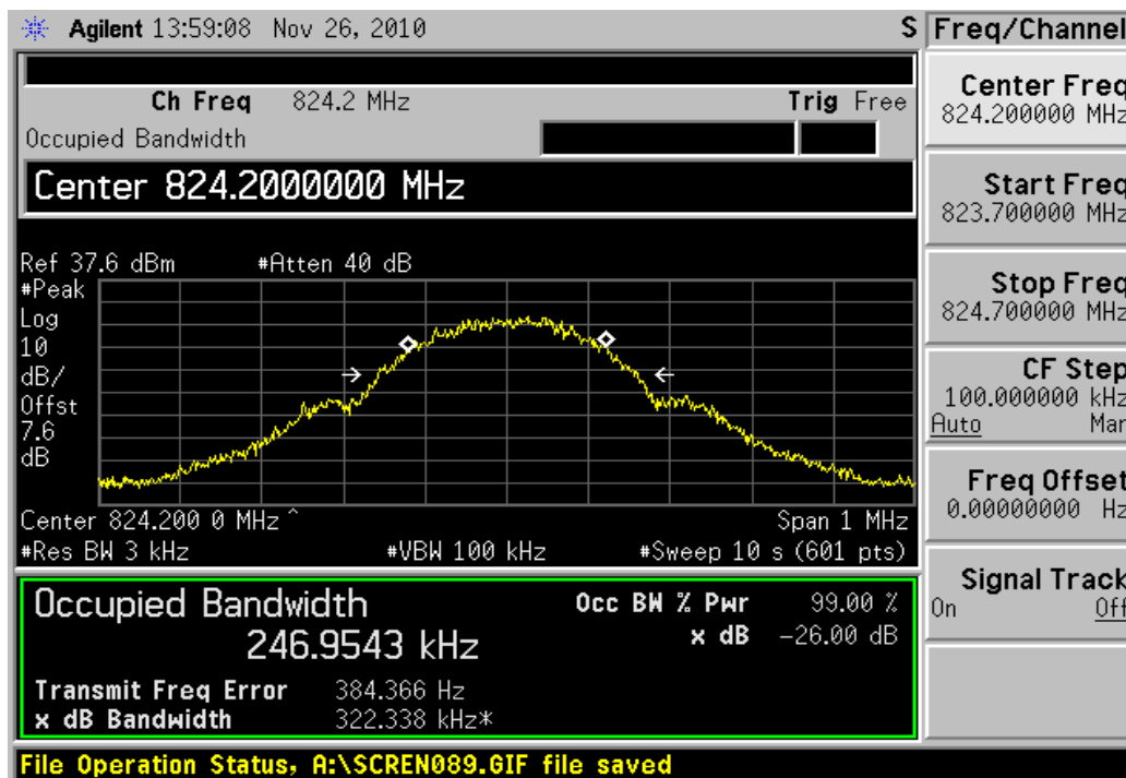
Channel 128
