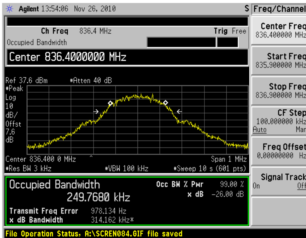
Channel 189
