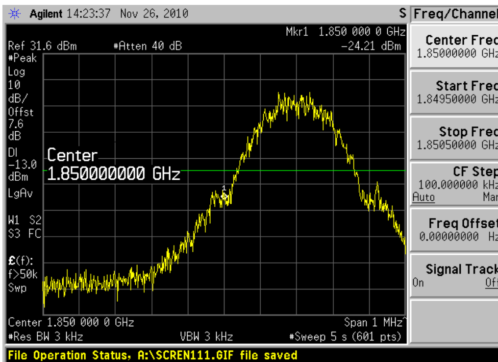
Channel 512
