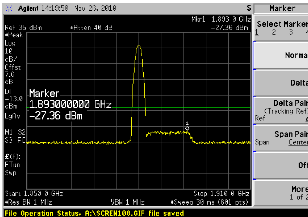
Channel 661, 1850MHz~1910MHz
