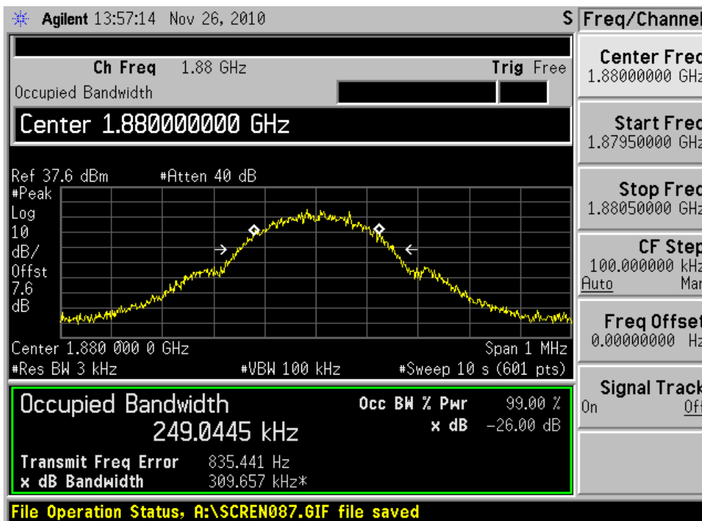
Channel 661
