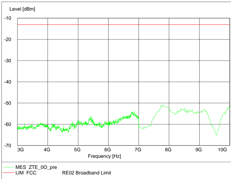
Channel 189, 3GHz~10GHz
