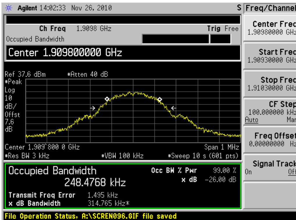
Channel 810
