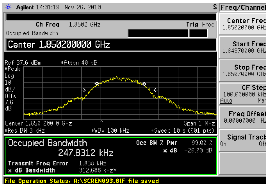
Channel 512
