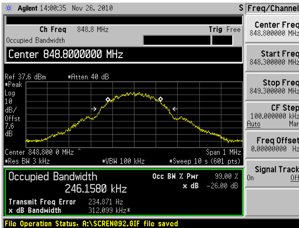
Channel 251
