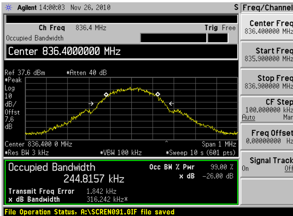
Channel 189
