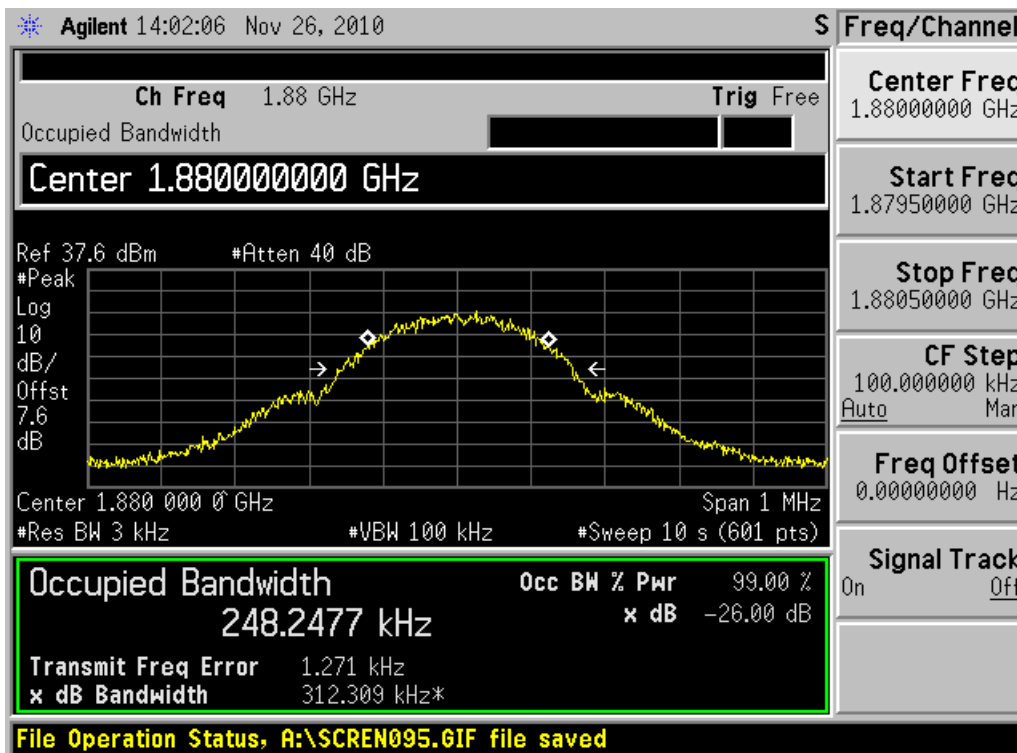
Channel 661
