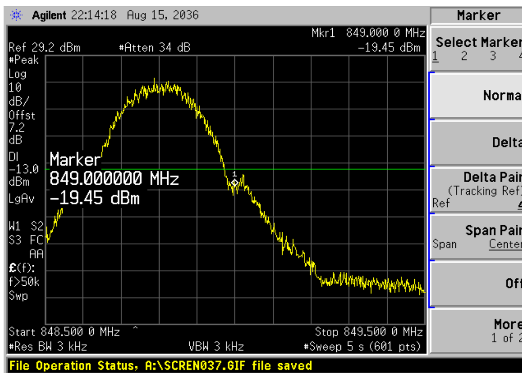
Channel 251
