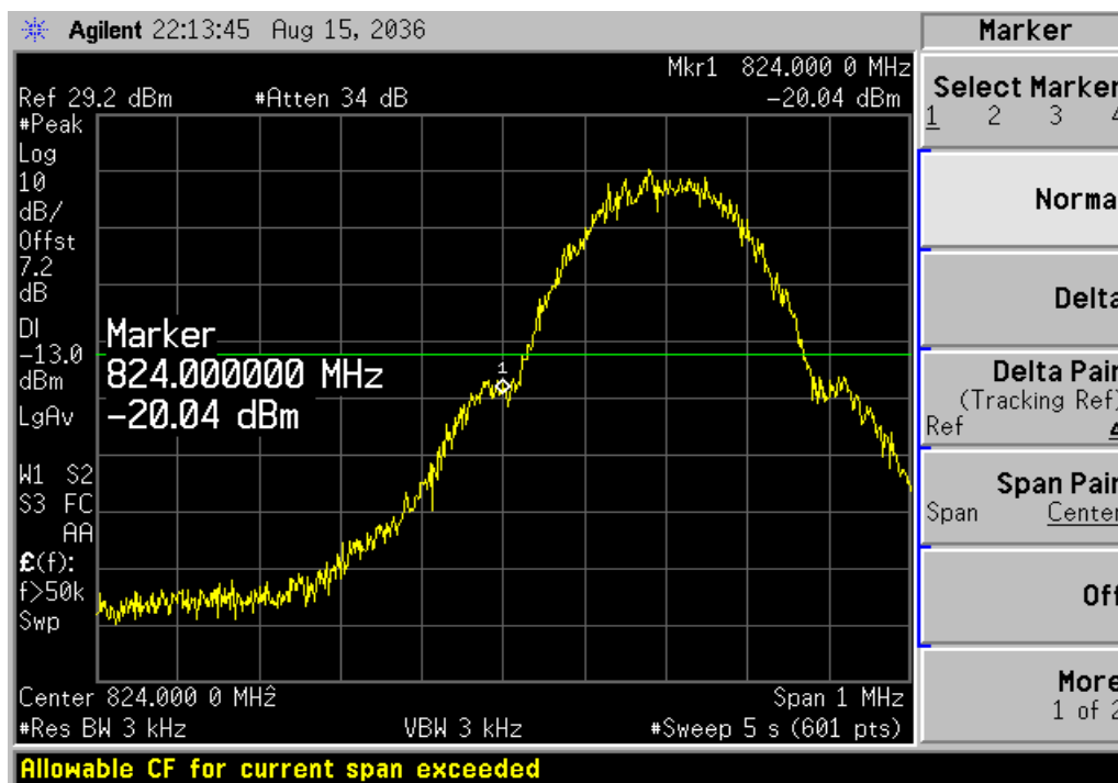
Channel 128
